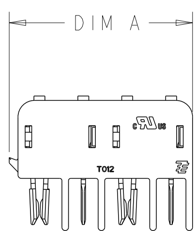
2058703-2/ 1-2078503-2 SCALE 3:1
