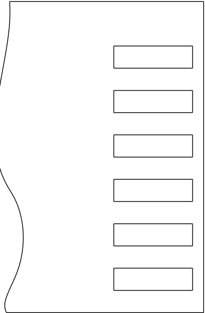
RECOMMENDED PCB LAYOUT FOR 2058703-3 & 1-2058703-3
