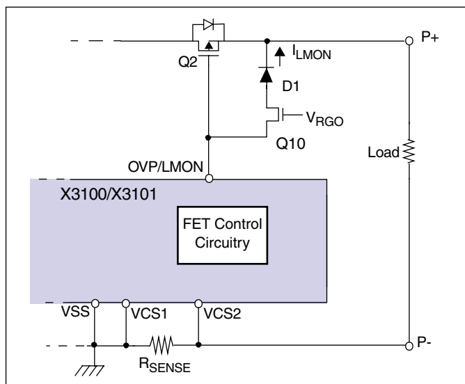
Figure 7. Over-Current Protection
