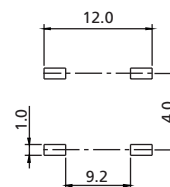
PCB LAYOUT
