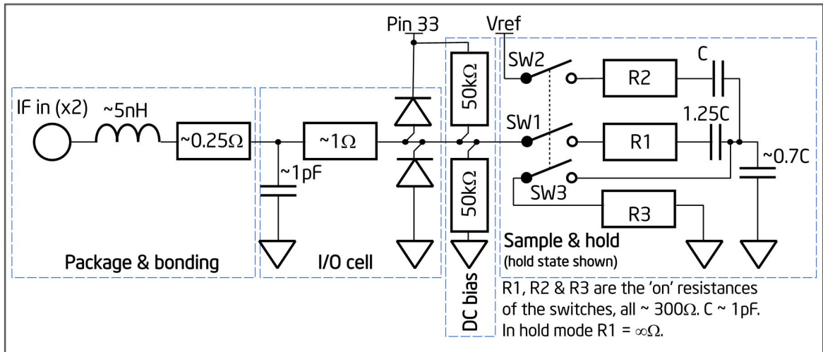
Figure 12 - VIN & VIN input impedance (approximate)
