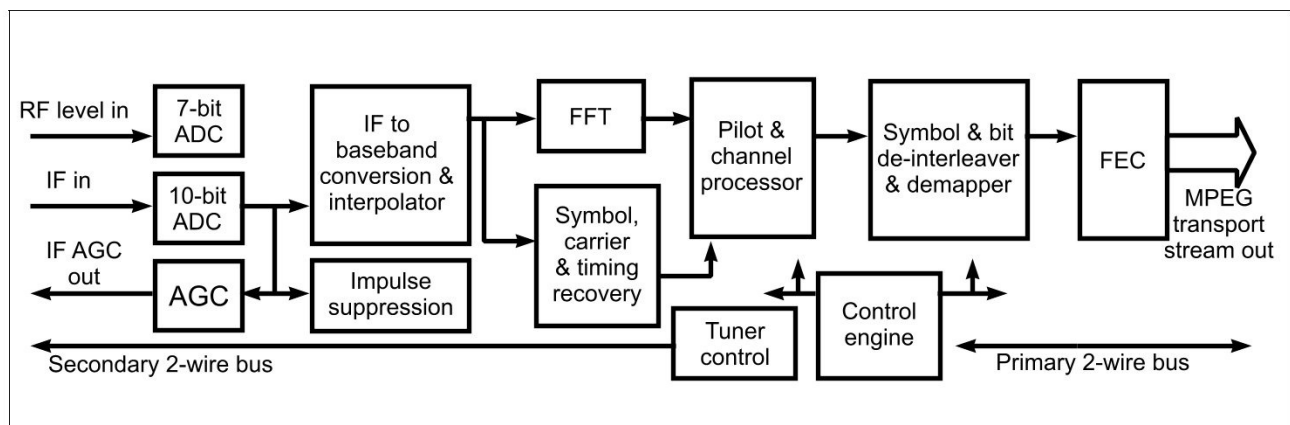
Figure 1- Block Diagram
