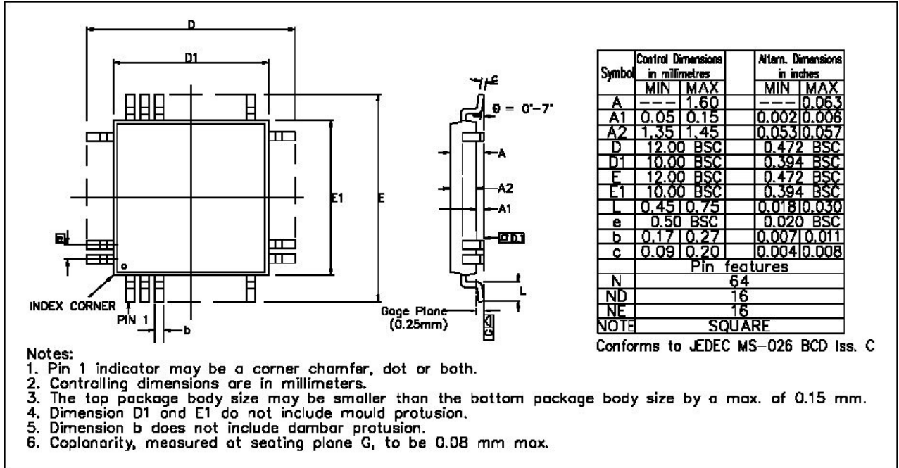
Figure 2 - Package dimensions
