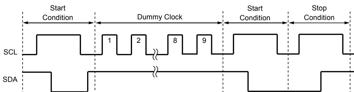
Figure 23 Resetting S-24C08C
