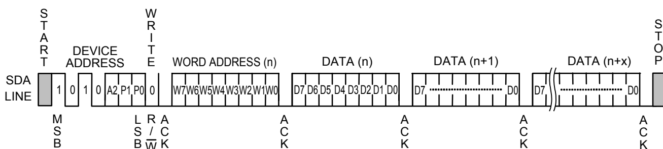
Figure 12 Page Write
