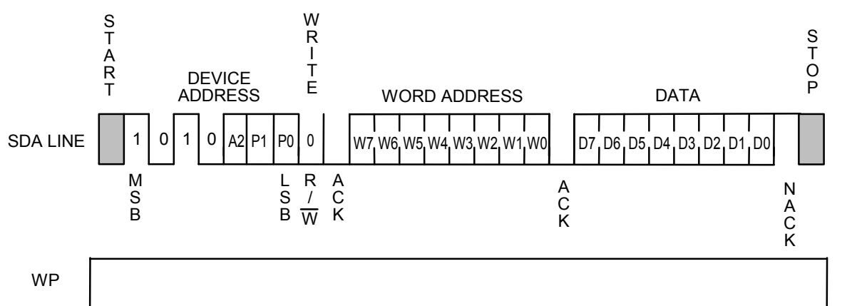
Figure 13 Write Protect
