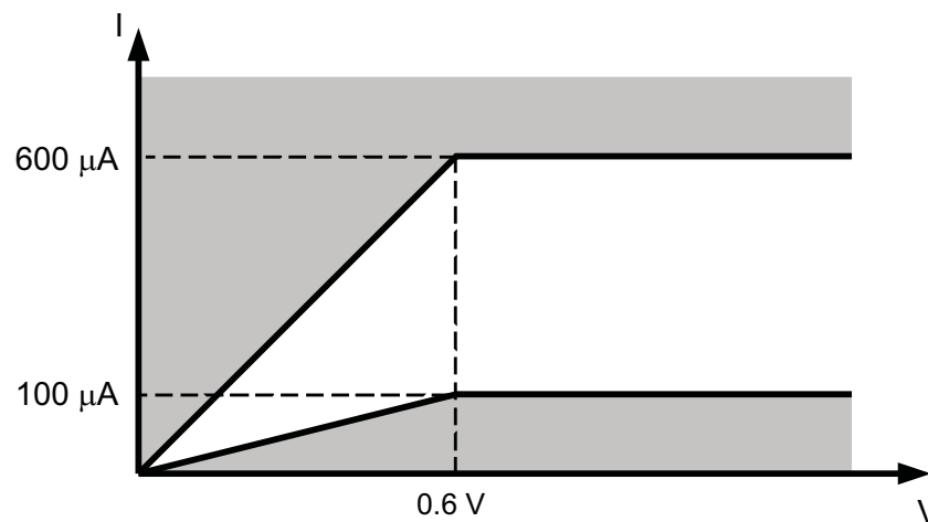
Figure 11. Microphone Current-to-Voltage Transfer Function
