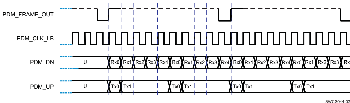
Figure 19. Normal Mode With Five Downlink and Two Uplink Channels Enabled
