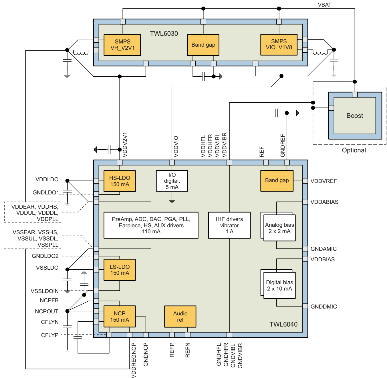
Figure 15. Power-Management Diagram
