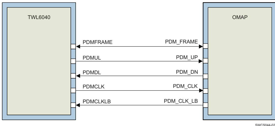
Figure 17. PDM Interface
