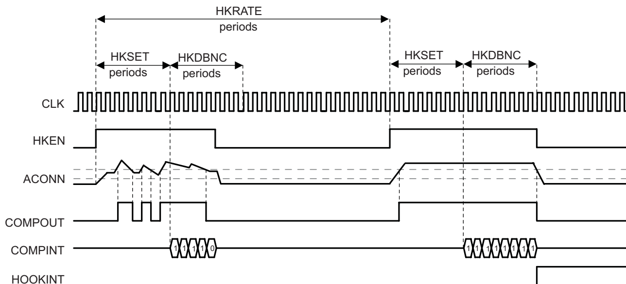
Figure 13. Detection Timing
