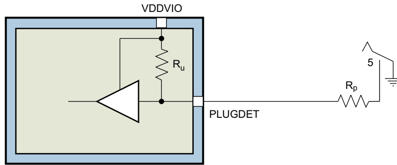
Figure 9. Plug Detection Circuit
