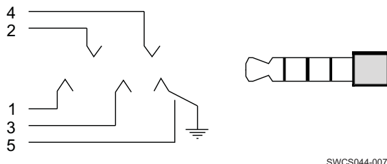
Figure 6. Standard Connector
