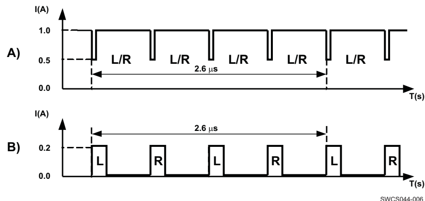
Figure 5. Current Load Waveforms, Worst-Case A) and Typical B)
