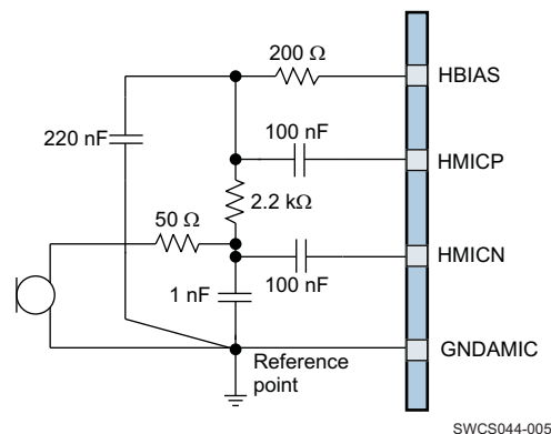
Figure 4. Board With Unavailable Negative Terminal
