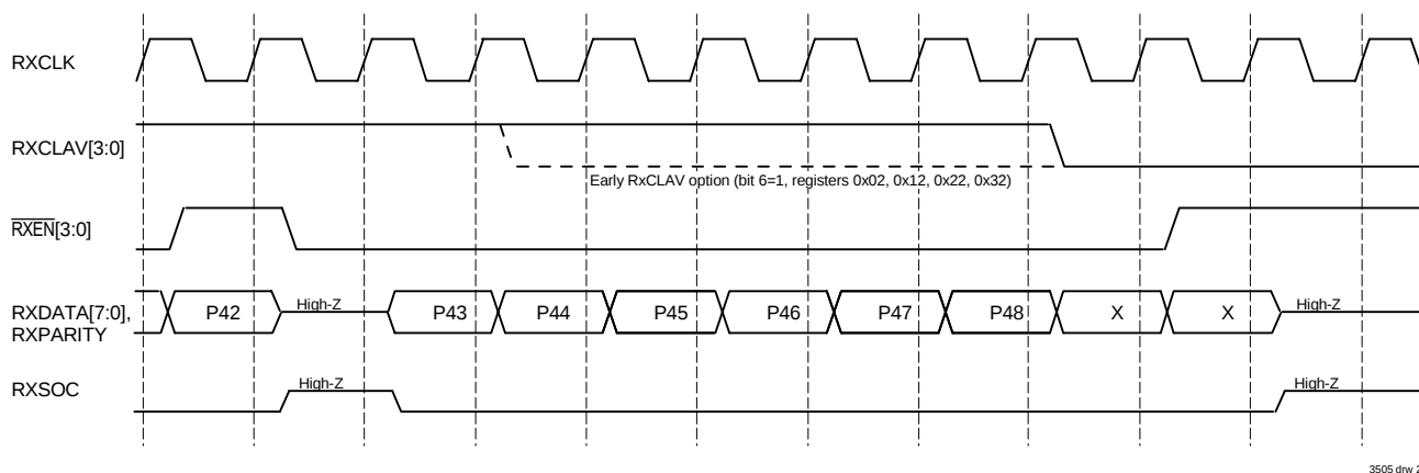
Figure 20 Utopia 1 Receive Handshake - RXCLAV Deassertion
