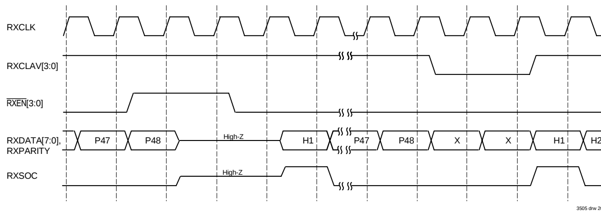
Figure 19 Utopia 1 Receive Handshake - \overline{\text{RXEN}} and RXCLAV Control
