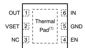
TPS728xx Series DRV PACKAGE 2mm x 2mm SON-6 (TOP VIEW)
