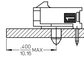
LOCATION DETAIL (SEE NOTE #6)
