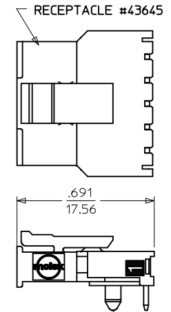
MATED MICRO FIT CONNECTOR
