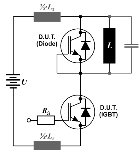
Figure E. Dynamic test circuit Leakage inductance L_\sigma = 180\text{nH} , and stray capacitance C_\sigma = 40\text{pF} .
