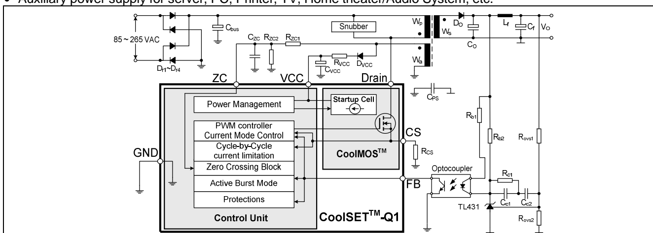
Figure 1 Typical Application
