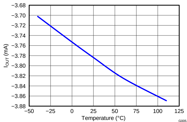
Figure 8. Output Current I_{OUT} vs. Temperature
