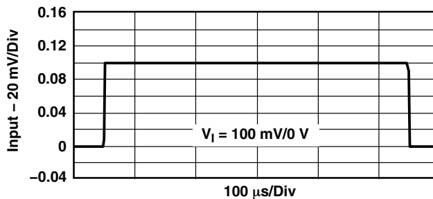
NONINVERTING SMALL-SIGNAL PULSE RESPONSE
