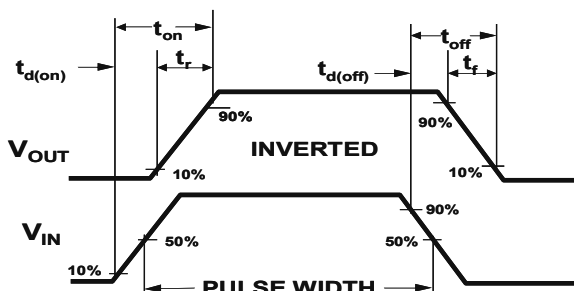
Figure 2: Switching Waveforms
