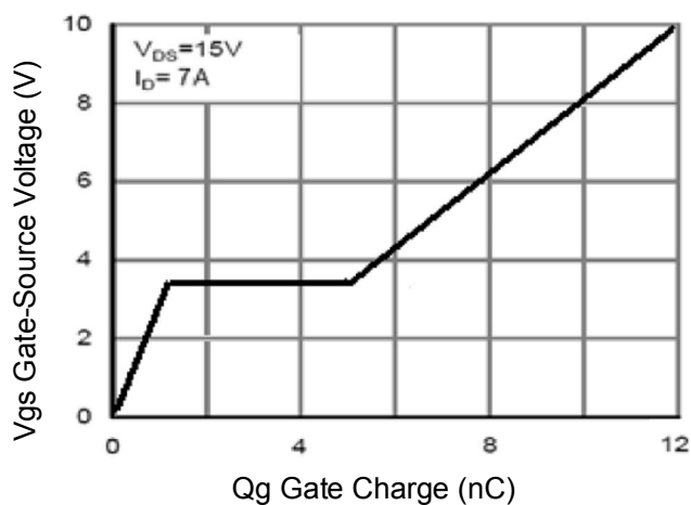
Figure 11 Gate Charge
