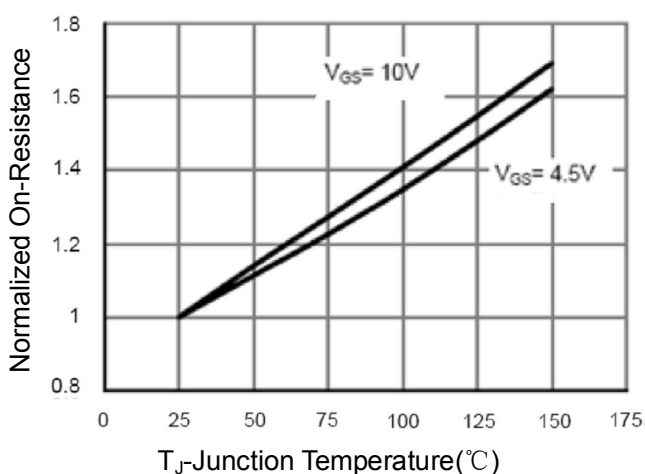
Figure 8 Drain-Source On-Resistance
