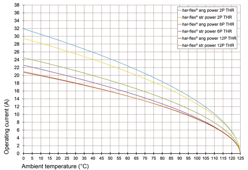
Derating curve 80%
