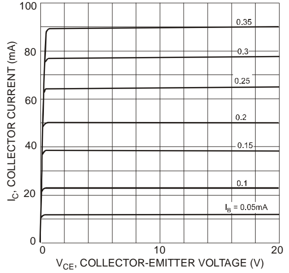
Figure 2 Typical Collector Current vs. Collector-Emitter Voltage
