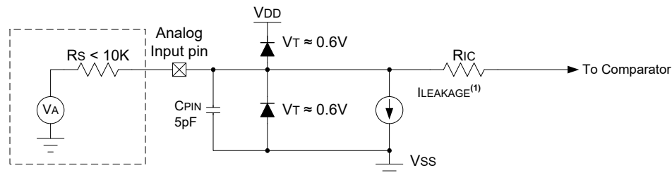
Figure 32-3. Analog Input Model
