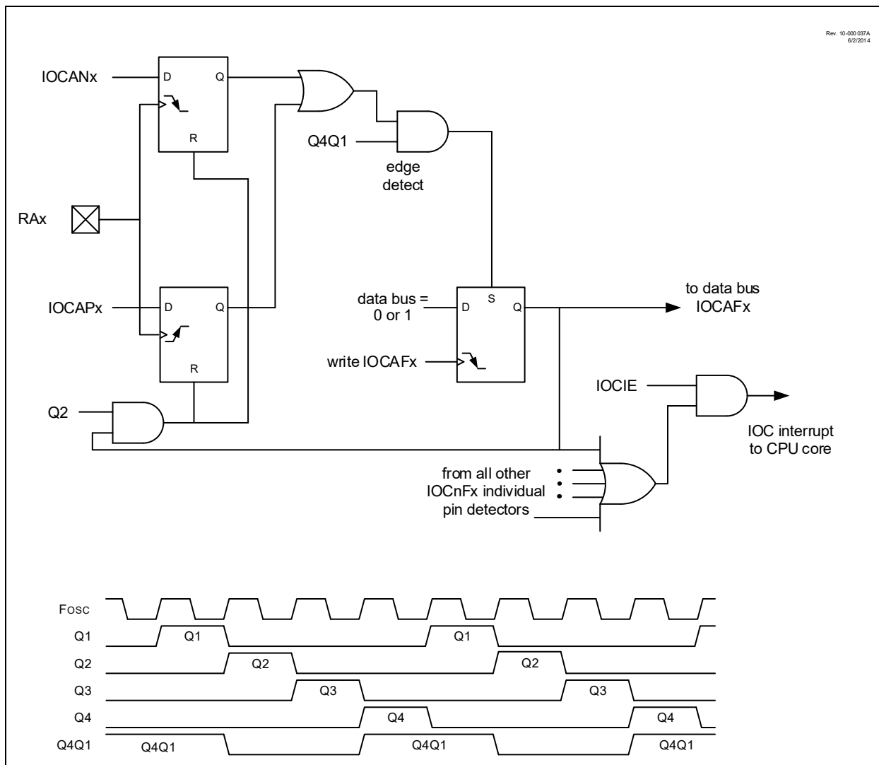
Figure 16-1. Interrupt-on-Change Block Diagram (PORTA Example)
