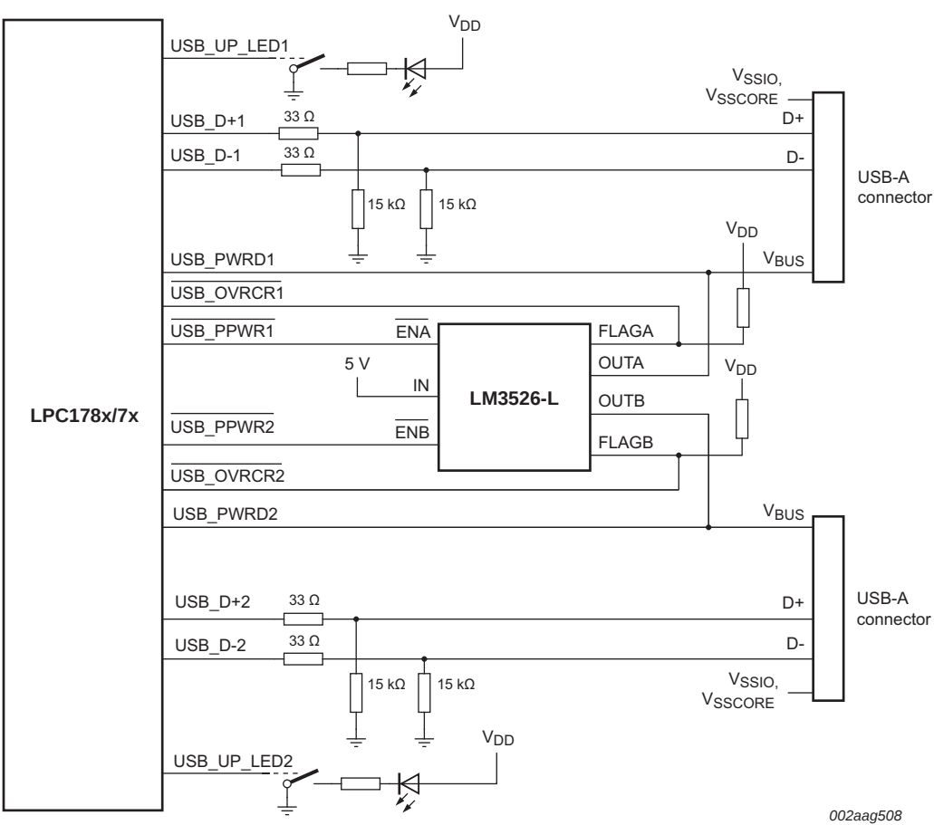
Fig 34. USB host port configuration: port 1 and port 2 as hosts
