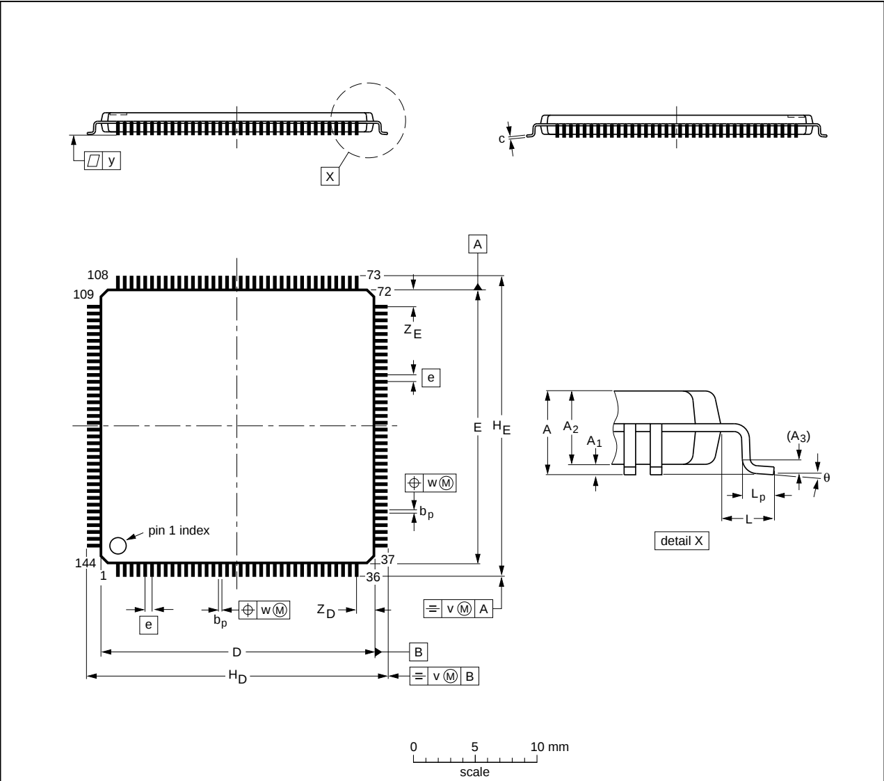
LQFP144: plastic low profile quad flat package; 144 leads; body 20 x 20 x 1.4 mm SOT486-1
