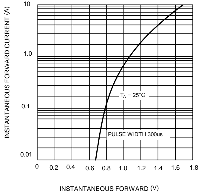
FIG.2-TYPICAL FORWARD CHARACTERISTICS
