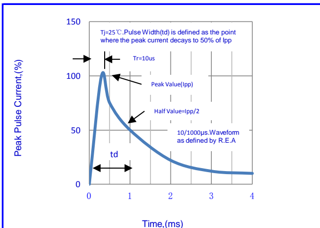
Fig.5-Pulse Waveform
