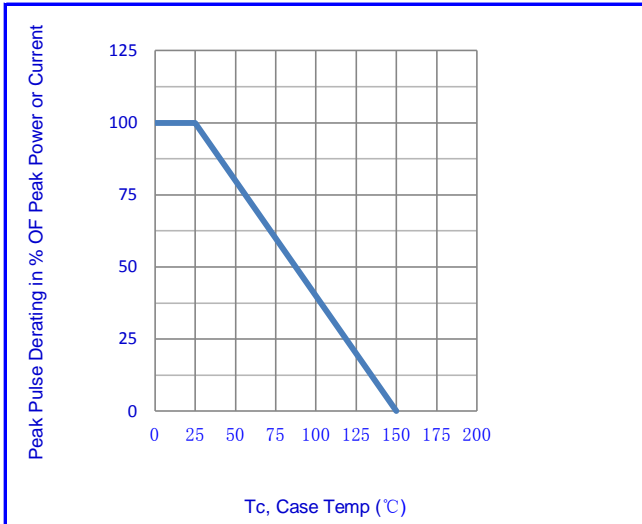
Fig.1-Pulse Derating Curve
