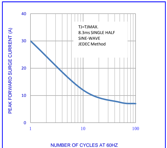
Fig.4-MAX. NON-REPETITIVE SURGE CURRENT
