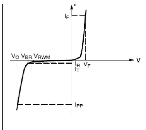
Figure 1. Uni-Directional TVS
