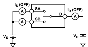
Figure 27. Off Leakage
