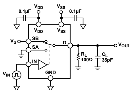
Figure 29. Switching Timing
