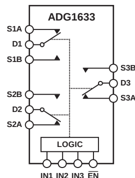
Figure 1. ADG1633 TSSOP and LFCSP
