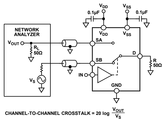
Figure 35. Channel-to-Channel Crosstalk
