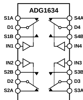
Figure 2. ADG1634 TSSOP
