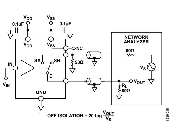
Figure 33. Off Isolation
