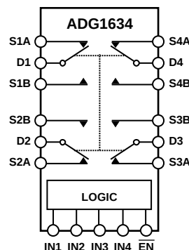
Figure 3. ADG1634 LFCSP
