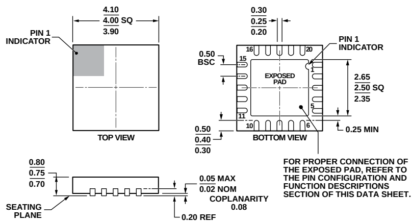
Figure 40. 20-Lead Lead Frame Chip Scale Package [LFCSP] 4 mm x 4 mm Body and 0.75 mm Package Height (CP-20-10)
