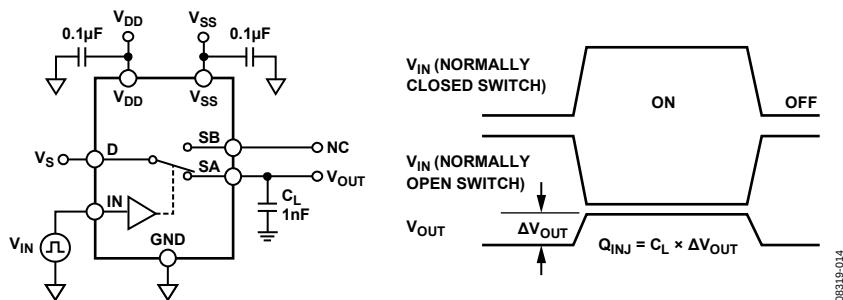
Figure 32. Charge Injection
