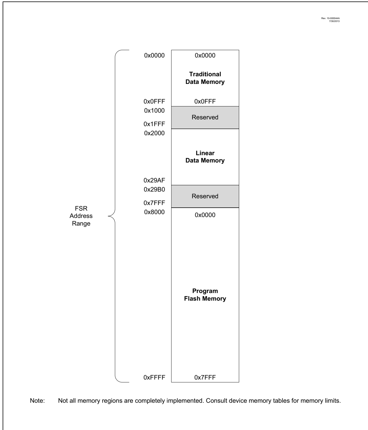
FIGURE 3-8: INDIRECT ADDRESSING
