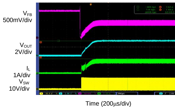
Over Voltage Recovery ( I_{OUT}=1.5\text{A} )
