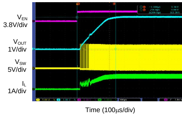
Enable Turn-on Characteristic (Resistance Load, R_{LOAD}=2.6\Omega )
