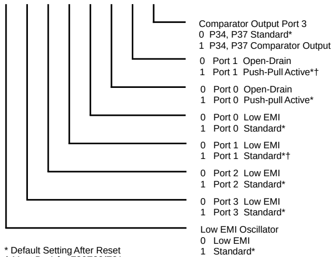
Figure 41. Port Configuration Register Write Only
