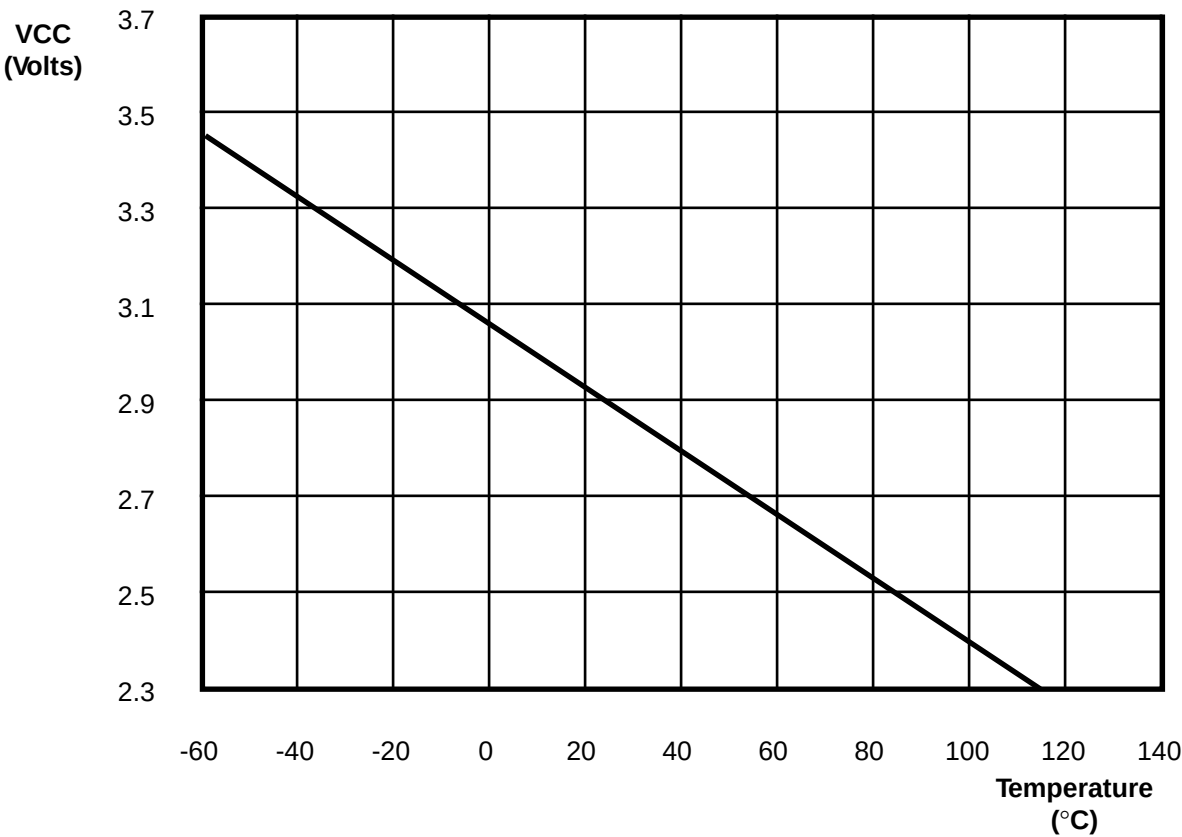
Figure 35. Typical Z86E40 V LV Voltage vs Temperature
