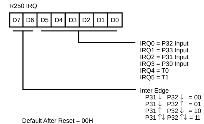
Figure 55. Interrupt Request Register FAH: Read/Write
