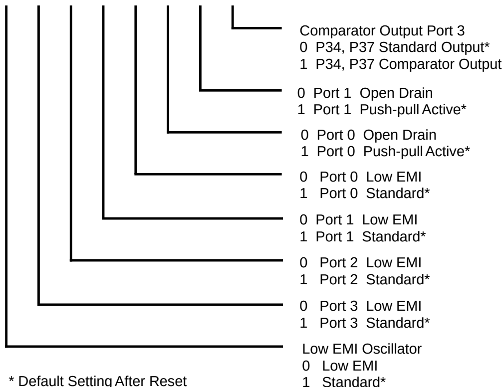
Figure 30. Port Configuration Register (PCON) (Write Only)
