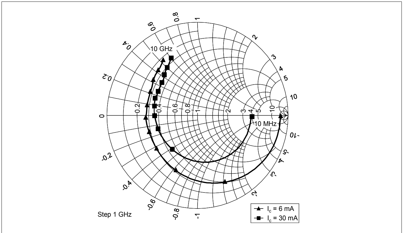
Figure 5-13 Input Matching S_{11} = f(f) , V_{CE} = 3 V, I_C = 6 / 30 mA
