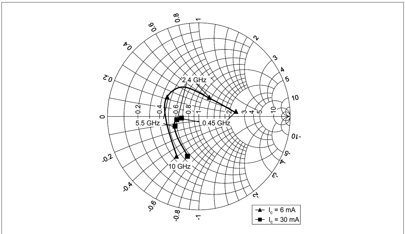
Figure 5-14 Source Impedance for Minimum Noise Figure Z_{opt} = f(f) , V_{CE} = 3 V, I_C = 6 / 30 mA
