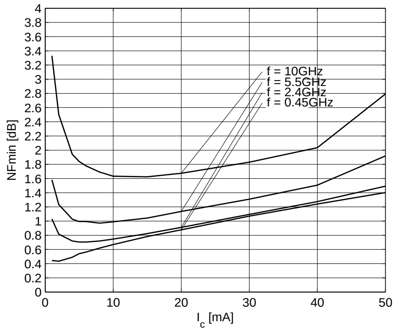
Figure 5-17 Noise Figure NF_{min} = f(I_c) , V_{CE} = 3\text{ V} , Z_S = Z_{opt} , f = \text{Parameter in GHz}
