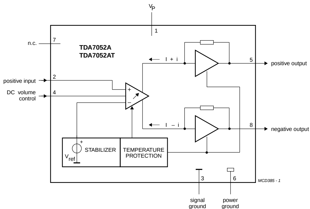
Fig.1 Block diagram.
