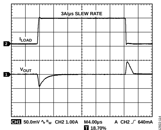
Figure 14. Load Transient Response, C_{OUT} = 10 μF, V_{IN} = 1.7 V, V_{OUT} = 1.3 V
