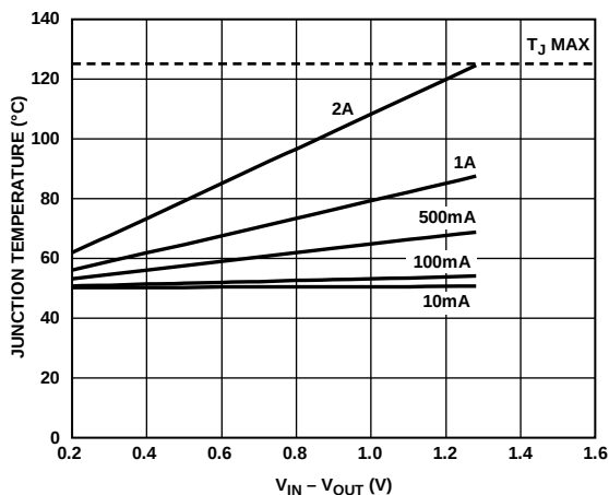
Figure 41. 500 mm² of PCB Copper, T_B = 50^\circ\text{C}
