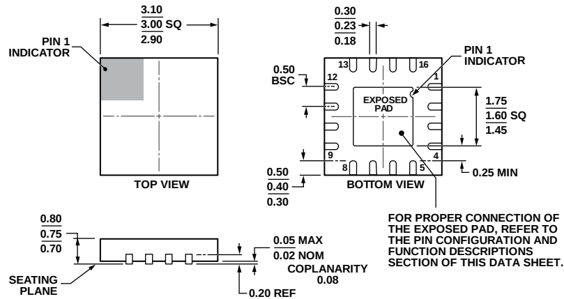
Figure 47. 16-Lead Lead Frame Chip Scale Package [LFCSP] 3 mm × 3 mm Body and 0.75 mm Package Height (CP-16-22) Dimensions shown in millimeters
