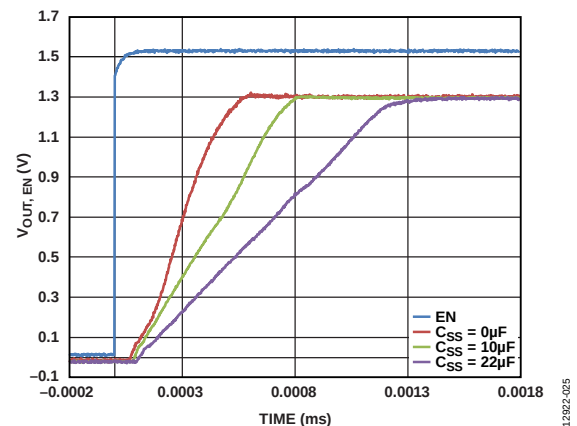
Figure 25. Fixed V_{\text{OUT}} Ramp-Up with External Soft Start Capacitor ( V_{\text{OUT, EN}} ) vs. Time
