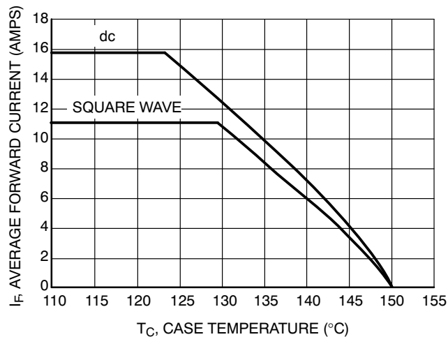
Figure 5. Current Derating
