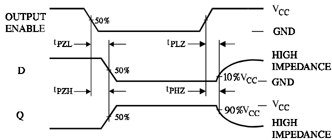
Figure 3. Switching Waveforms
