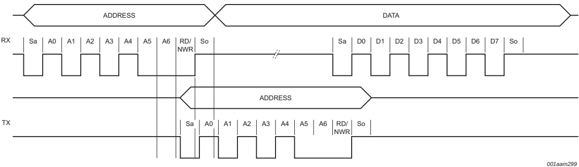
Fig 15. Timing diagram for UART write data
