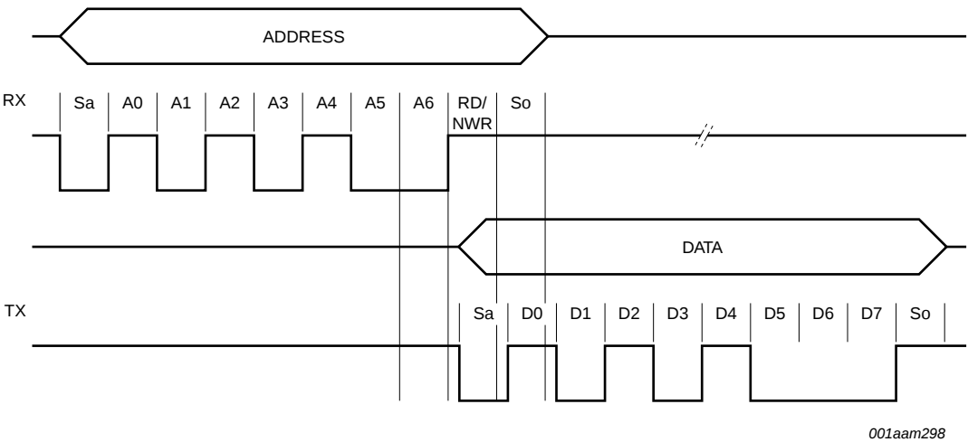
Fig 14. Timing Diagram for UART Read Data
