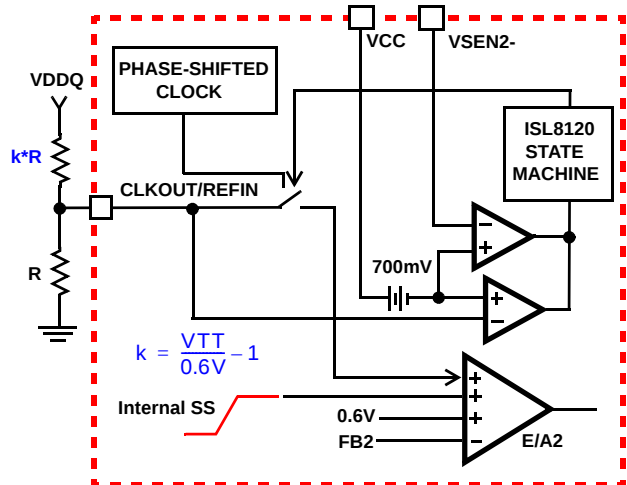
FIGURE 25. SIMPLIFIED DDR IMPLEMENTAION
