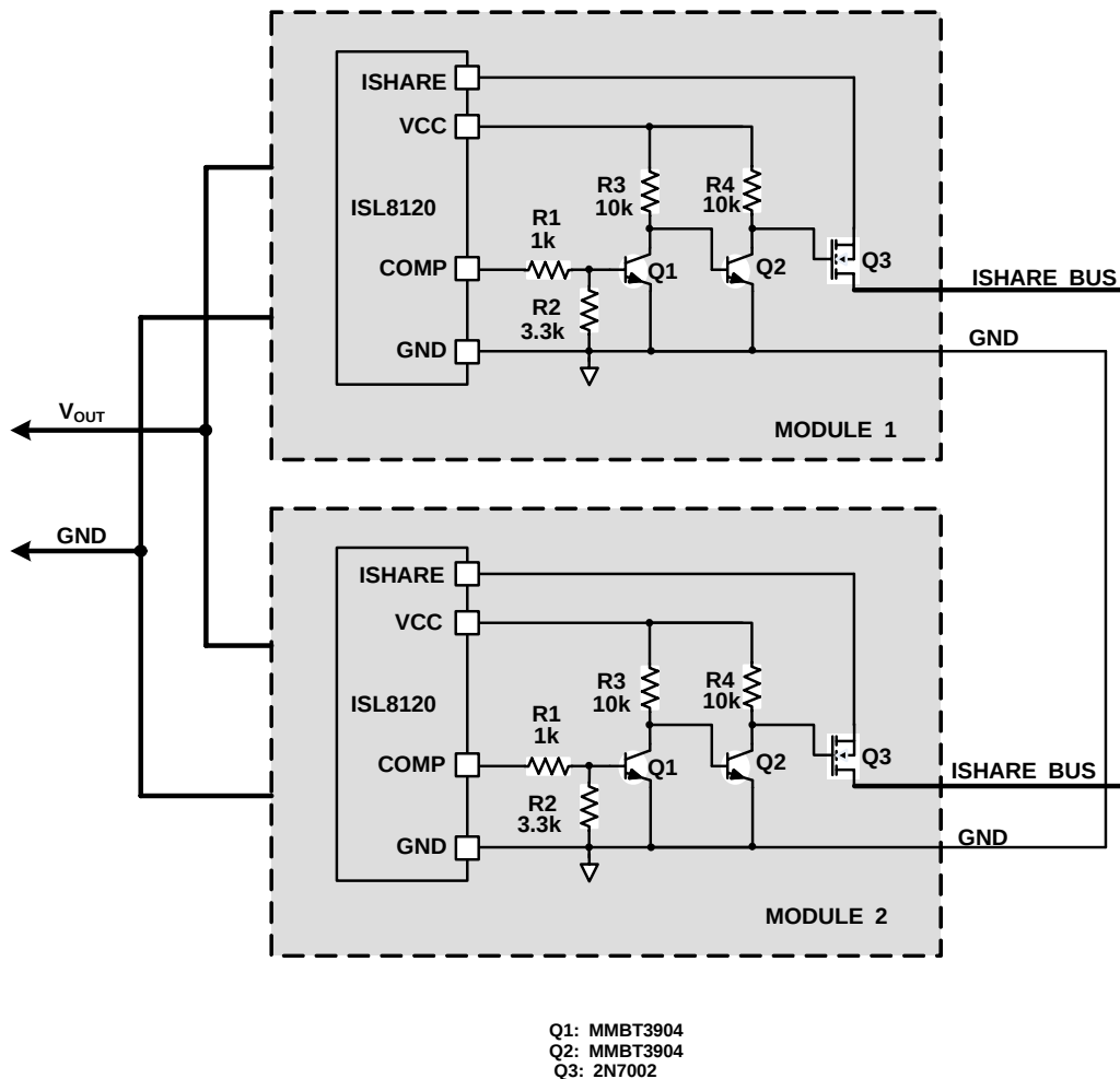
FIGURE 15. SINGLE COMMUNICATION WIRE CONNECTION
