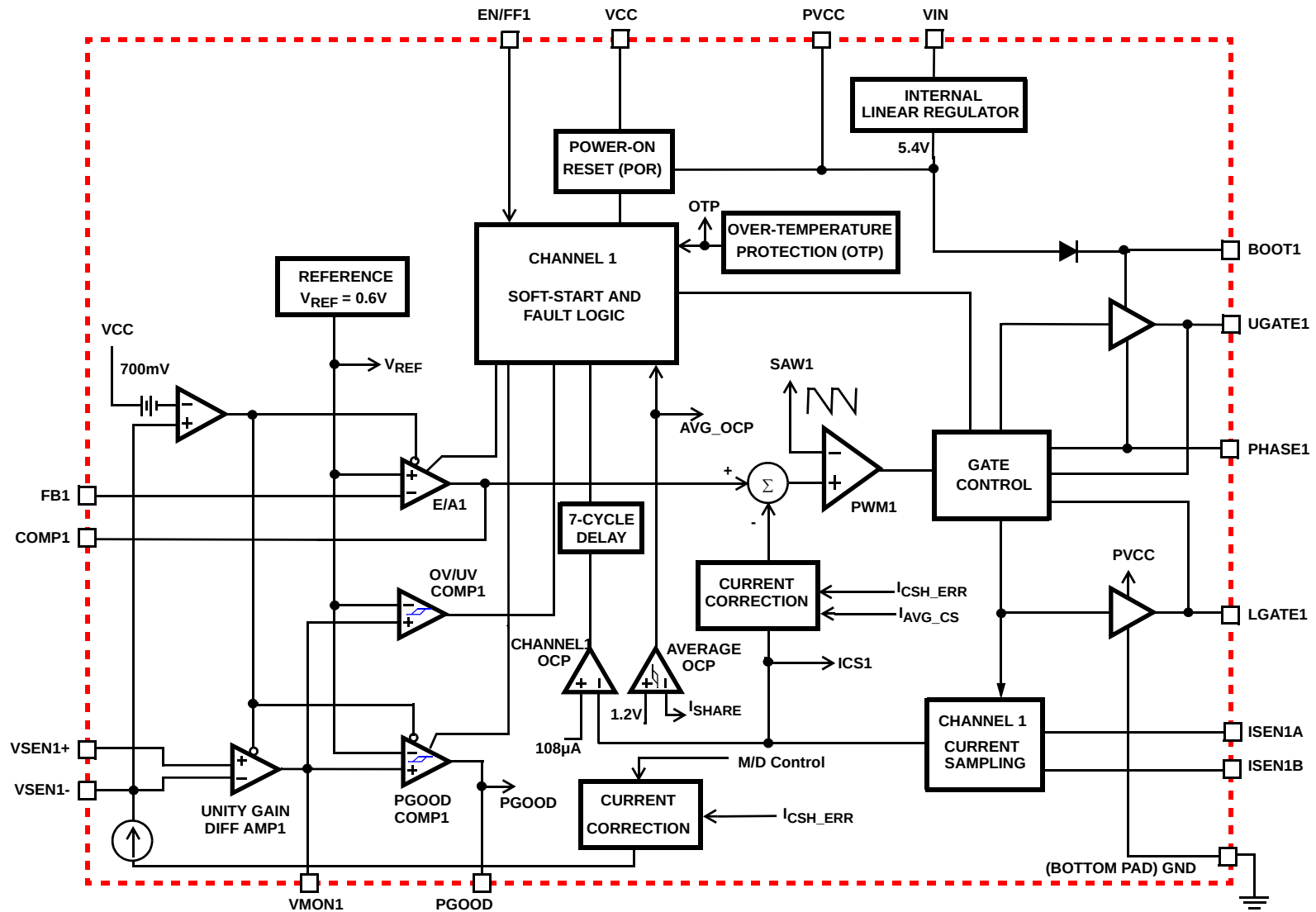
FIGURE 1. CHANNEL/PHASE 1 (VDDQ)
