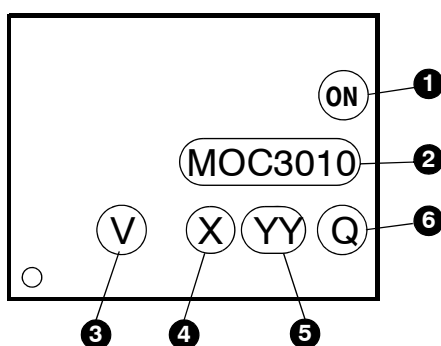
Figure 14. Top Marking
