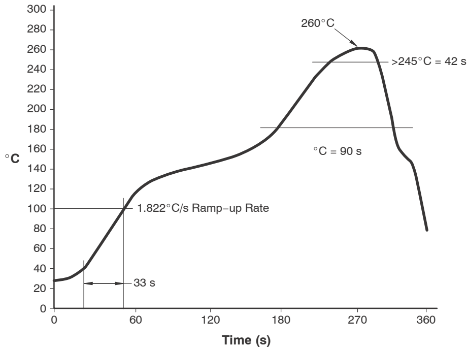
Figure 13. Reflow Profile
