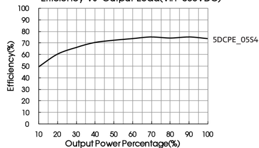
Efficiency Vs Output Load(Vin=500VDC)
