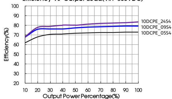
Efficiency Vs Output Load(Vin=500VDC)
