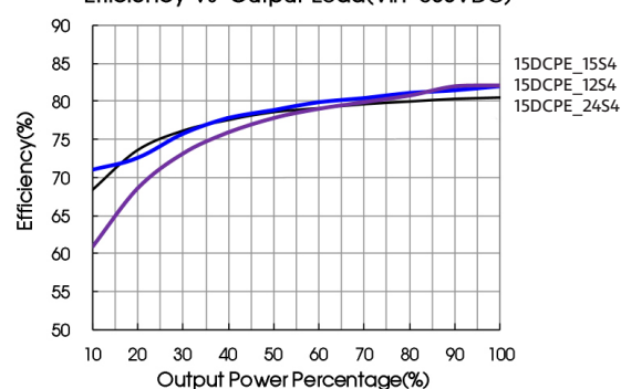
Efficiency Vs Output Load(Vin=500VDC)
