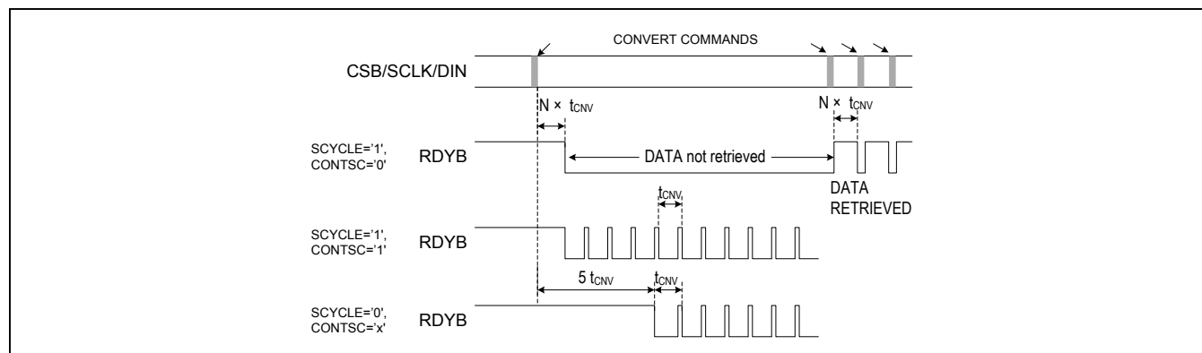
Figure 4. Timing of RDYB in All Conversion Configurations: Single-Cycle, Single-Cycle Continuous, and Continuous. In sequencer mode 1 and in sequencer modes 2 and 3, with SEQ:RDYBEN='0' N = 1 . In sequencer modes 2 and 3 with SEQ:RDYBEN='1' N = number of active channels.
