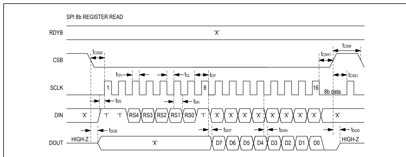
Figure 7. SPI Register Read Timing Diagram. For read patterns, the user may latch the MAX11253 output data on either rising edges (9–16) running at minimum latency or falling edges 9–16 running at increased latency.
