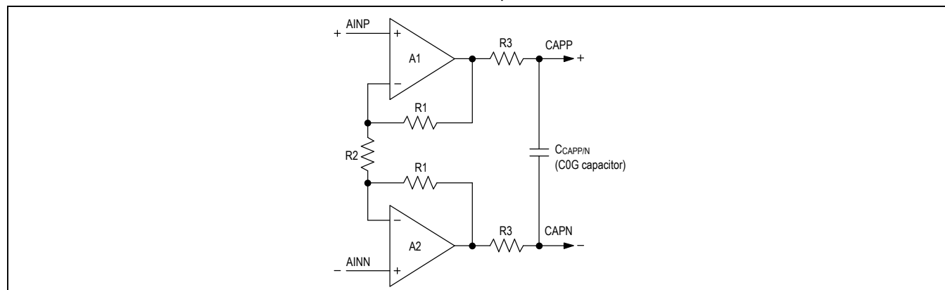
Figure 2. Simplified Equivalent Diagram of the PGA
