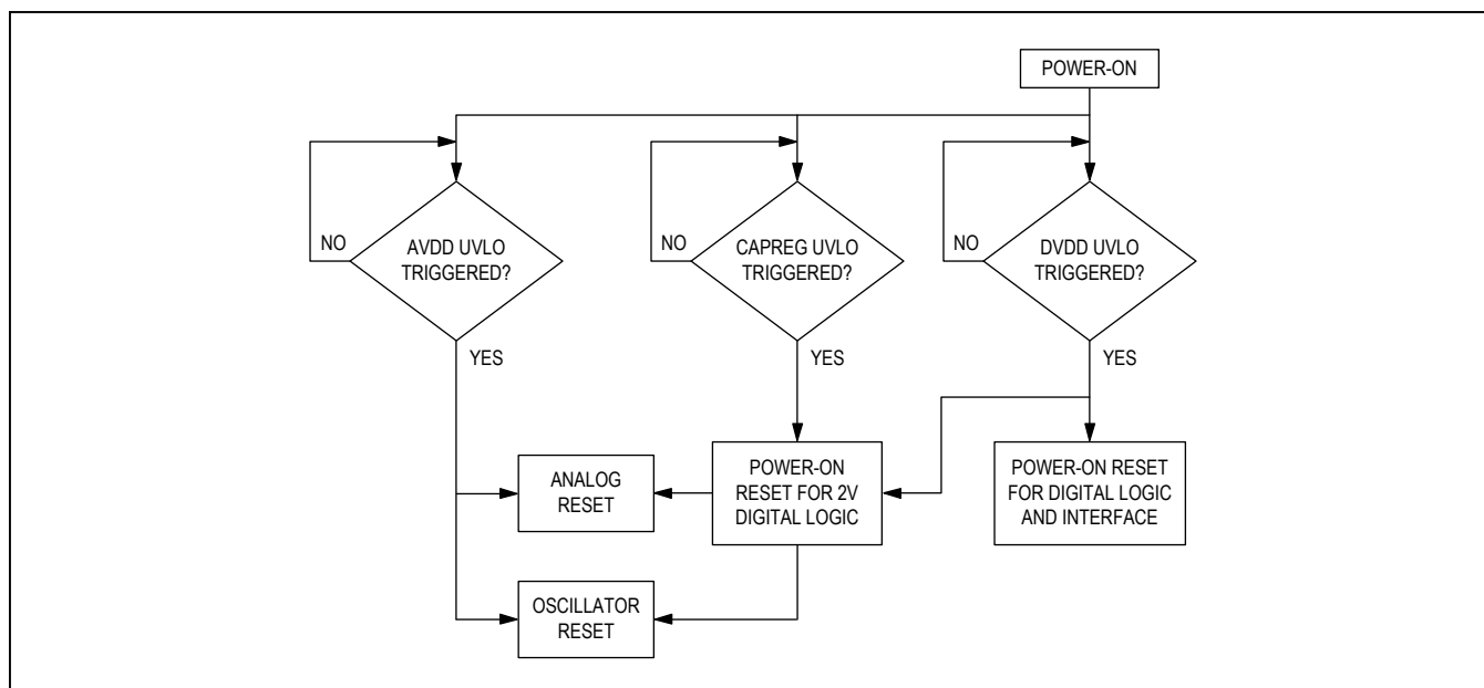
Figure 14. MAX11253 UVLO and POR Flow Diagram
