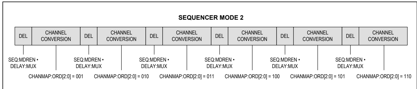
Figure 10. Sequencer Mode 2 Timing Diagram
