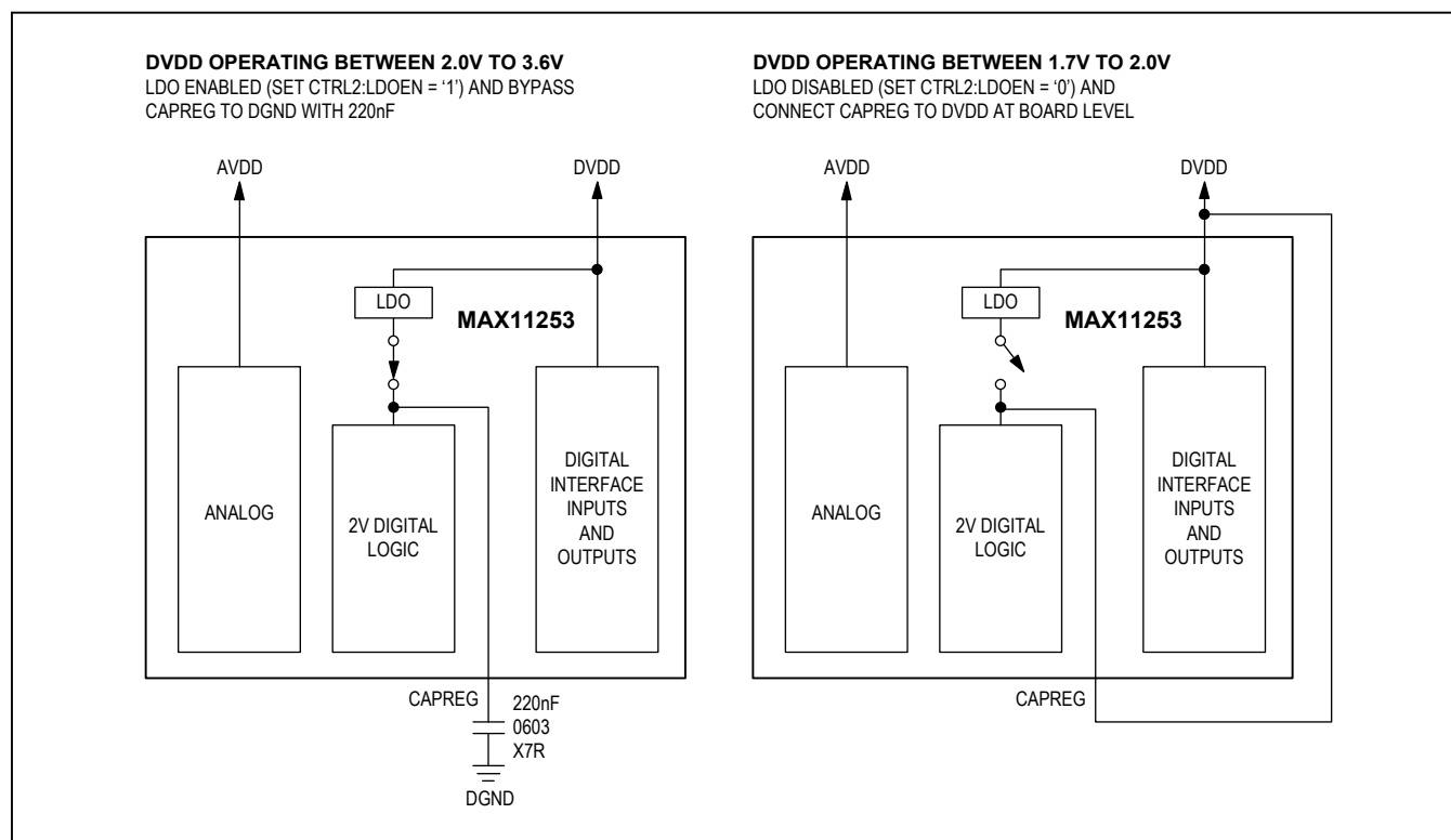
Figure 12. MAX11253 Digital Power Architecture
