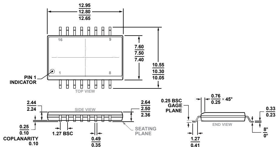
Figure 28. 16-Lead Standard Small Outline Package, with Increased Creepage [SOIC_IC] Wide Body (RI-16-2)
