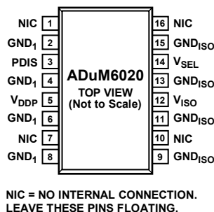
Figure 5. Pin Configuration
