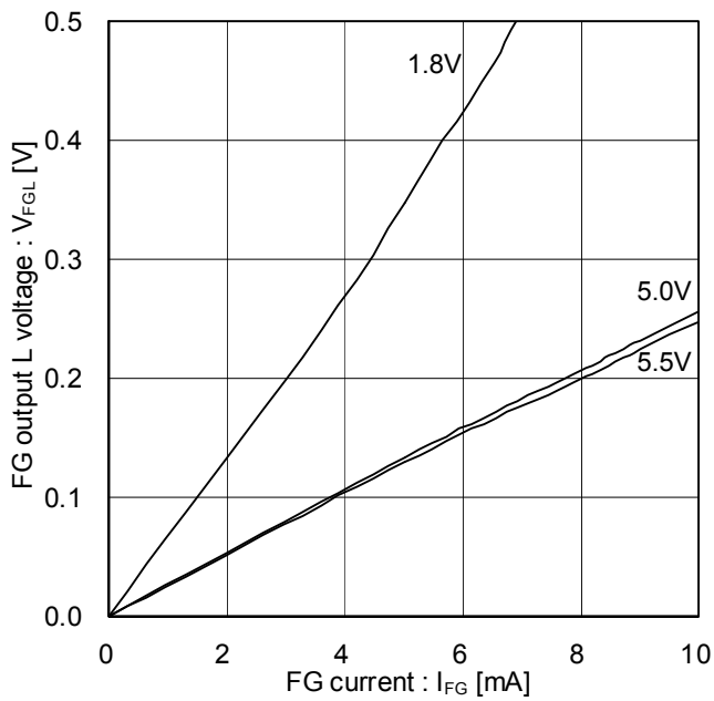
Figure 15. FG Output L Voltage (Voltage Characteristics)
