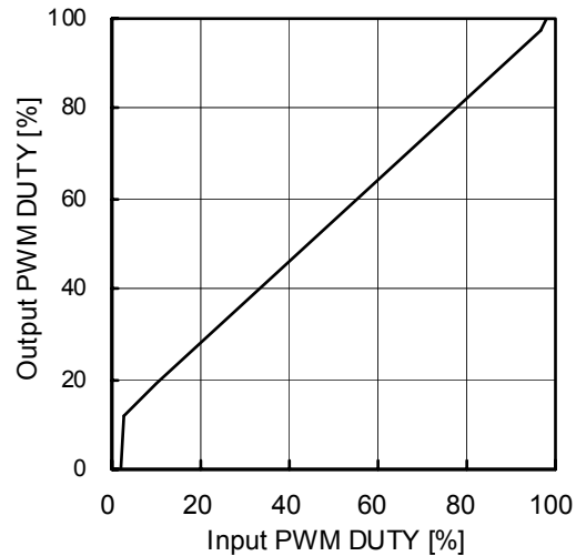
Figure 21. Characteristic of input PWM DUTY and output PWM DUTY
