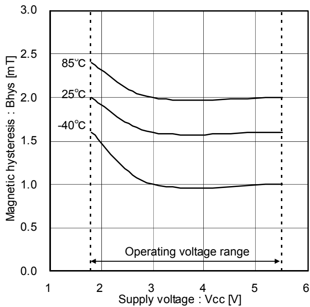
Figure 7. Magnetic hysteresis
