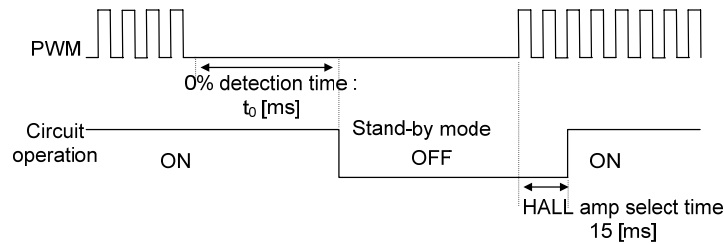
Figure 24. Stand-by mode and quick start function
