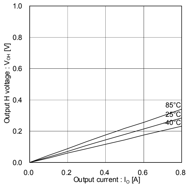
Figure 8. Output H Voltage (Temperature Characteristics)
