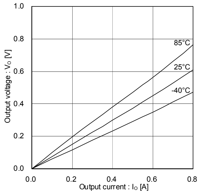
Figure 12. Total Output Voltage (Output H and L) (Temperature Characteristics)
