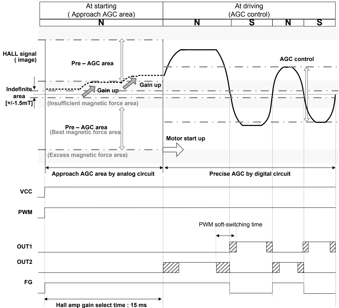
Figure 19. AGC Image of the Hall signal (In case of weak magnetic field)
