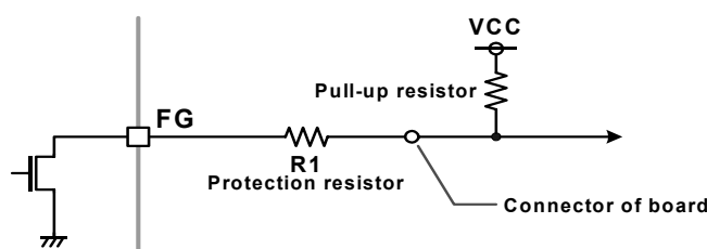
Figure 31. Protection of FG terminal
