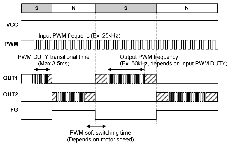
Figure 22. Timing chart of PWM control
