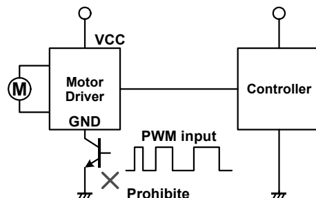
Figure 30. GND Line PWM switching prohibited
