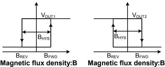
Figure 2. Output operation
