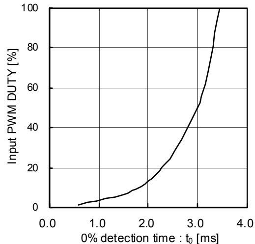
Figure 25. Characteristic curve of 0% detection time and input PWM duty at 25kHz
