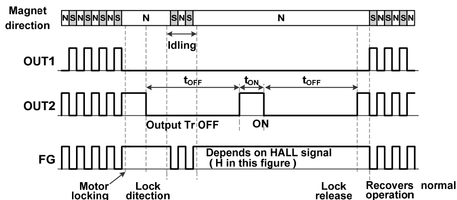
Figure 26. Lock protection timing chart
