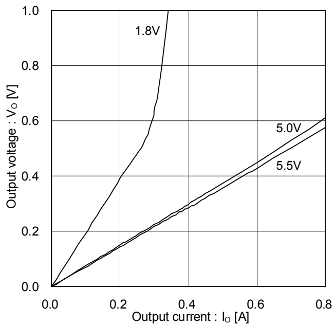
Figure 13. Total Output Voltage (Output H and L) (Voltage Characteristics)
