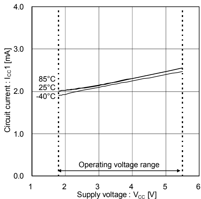
Figure 3. Circuit Current 1
