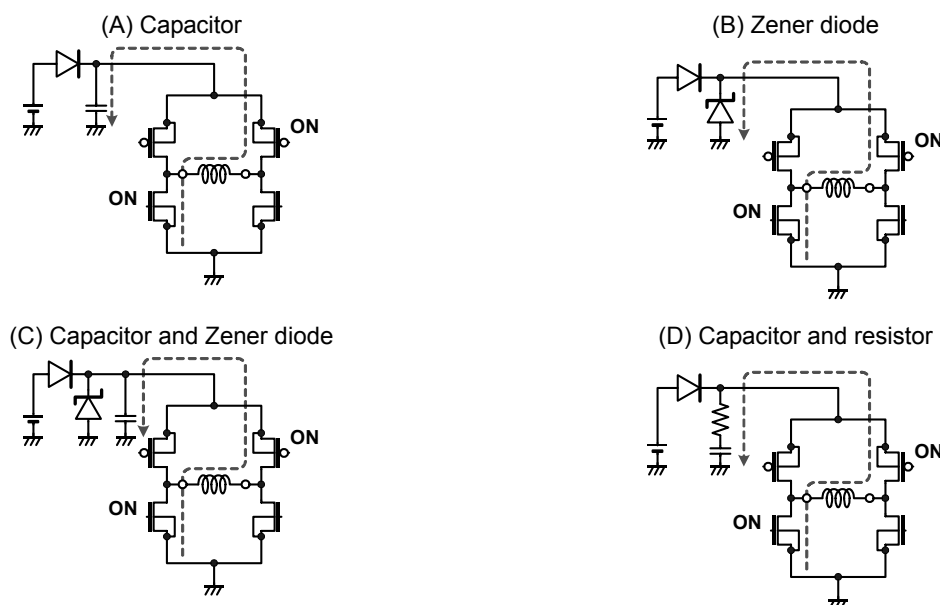
Figure 29. Protection against VCC voltage rise
