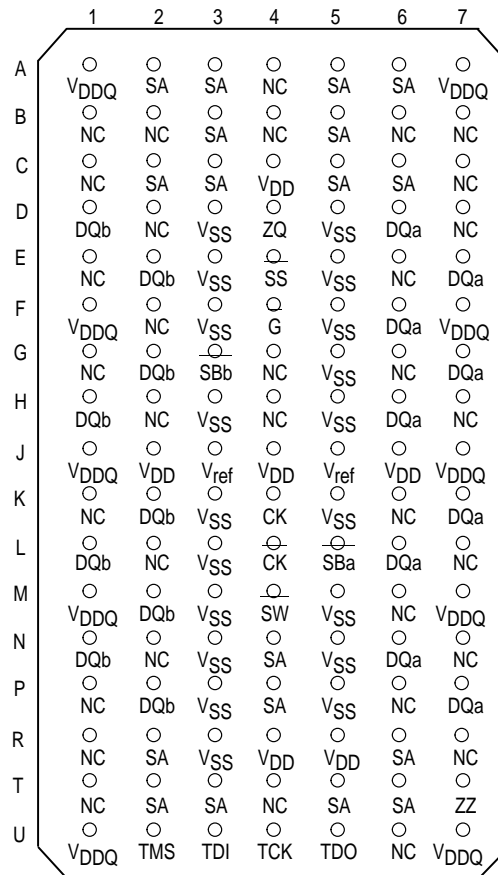
MCM69R818A
