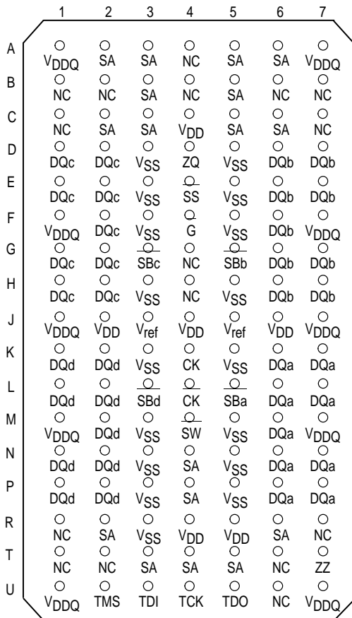
MCM69R736A
