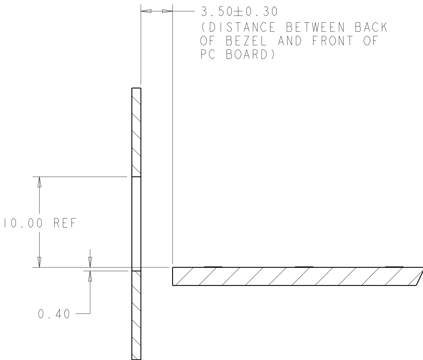
SECTION X-X
