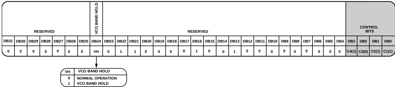
Figure 39. Register 11
