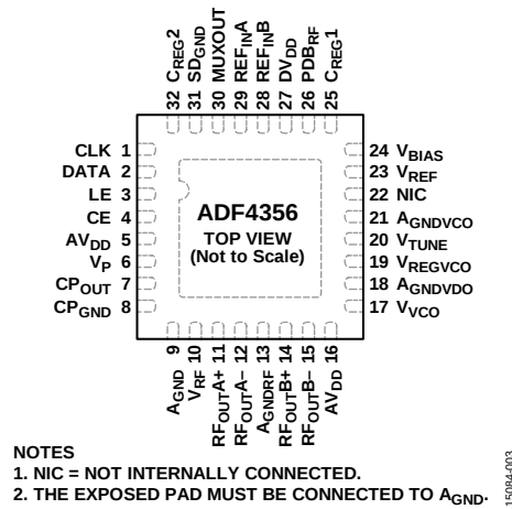
Figure 3. Pin Configuration
