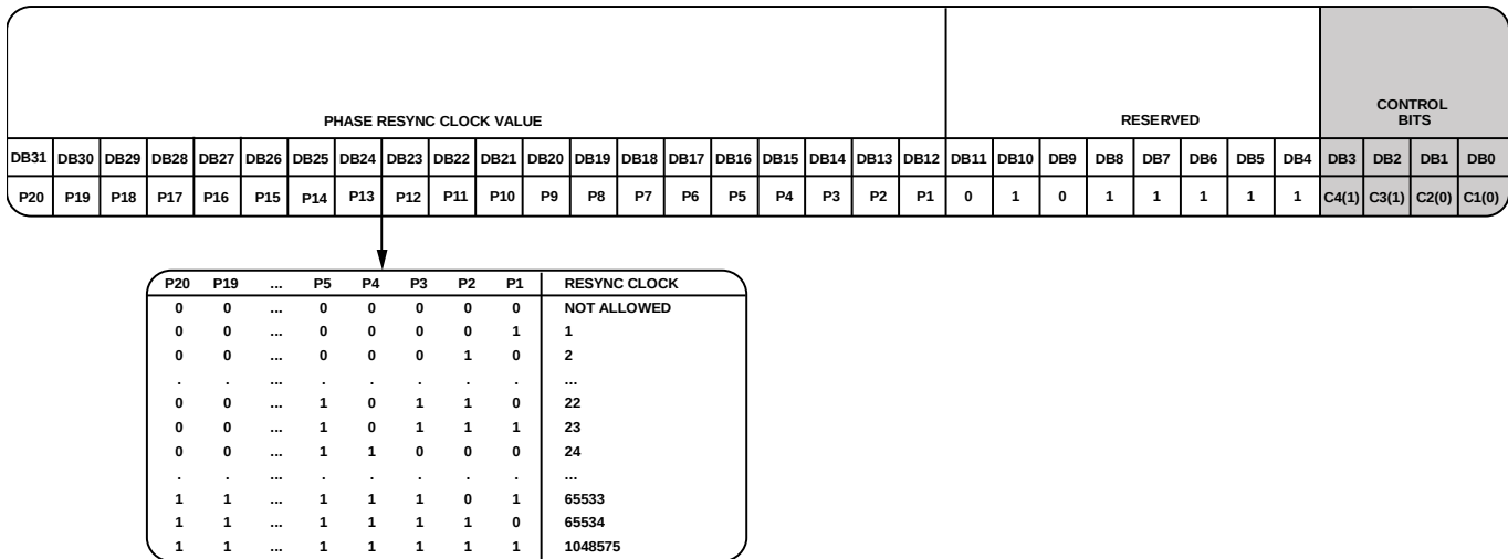
Figure 40. Register 12
