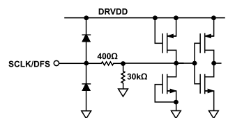
Figure 47. Equivalent SCLK/DFS Input Circuit
