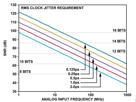
Figure 62. Ideal SNR vs. Input Frequency and Jitter
