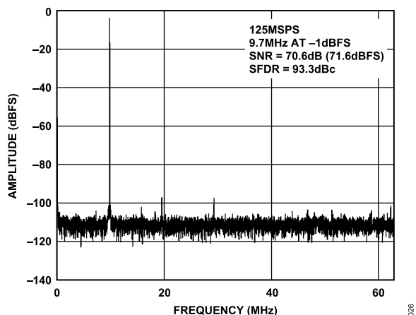
Figure 26. Single-Tone 16k FFT with f_{IN} = 9.7 MHz, f_{SAMPLE} = 125 MSPS
