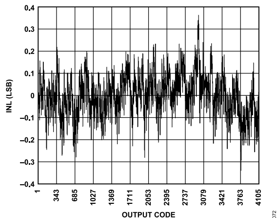
Figure 37. INL; f_{IN} = 9.7 MHz, f_{SAMPLE} = 125 MSPS
