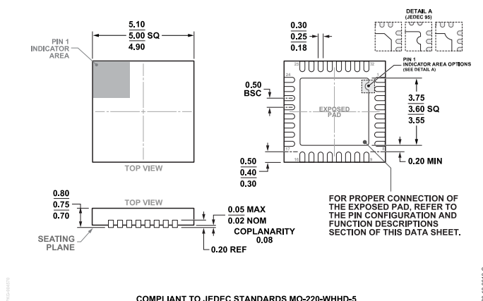
Figure 70. 32-Lead Lead Frame Chip Scale Package [LFCSP] 5 mm x 5 mm Body and 0.75 mm Package Height (CP-32-12) Dimensions shown in millimeters
