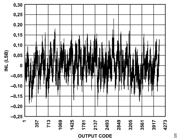
Figure 20. INL; f_{IN} = 9.7 MHz, f_{SAMPLE} = 80 MSPS
