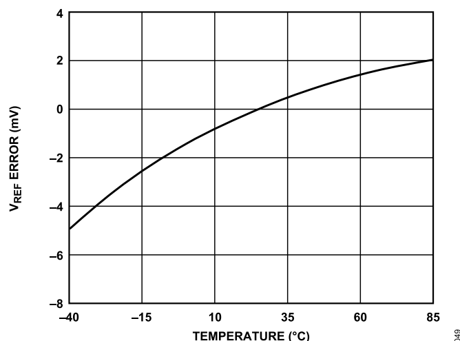
Figure 54. Typical V_{\text{REF}} Drift
