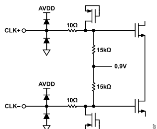
Figure 44. Equivalent Clock Input Circuit
