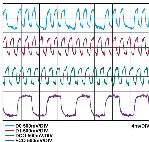
Figure 64. AD9635-125, LVDS Output Timing Example in ANSI-644 Mode (Default)
