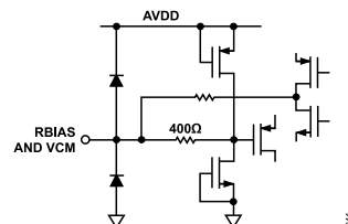
Figure 48. Equivalent RBIAS and VCM Circuit
