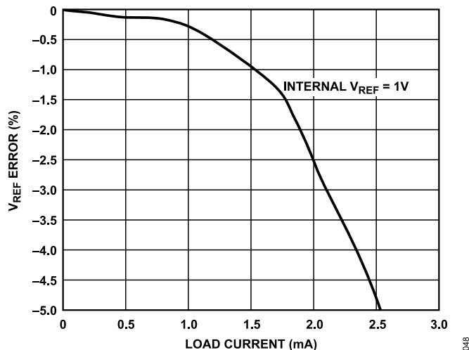
Figure 53. V_{\text{REF}} Error vs. Load Current
