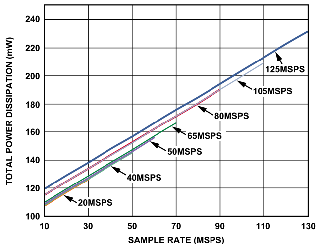
Figure 63. Total Power Dissipation vs. f_{\text{SAMPLE}} for f_{\text{IN}} = 9.7 \text{ MHz}
