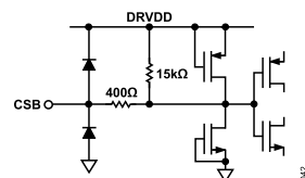
Figure 49. Equivalent CSB Input Circuit
