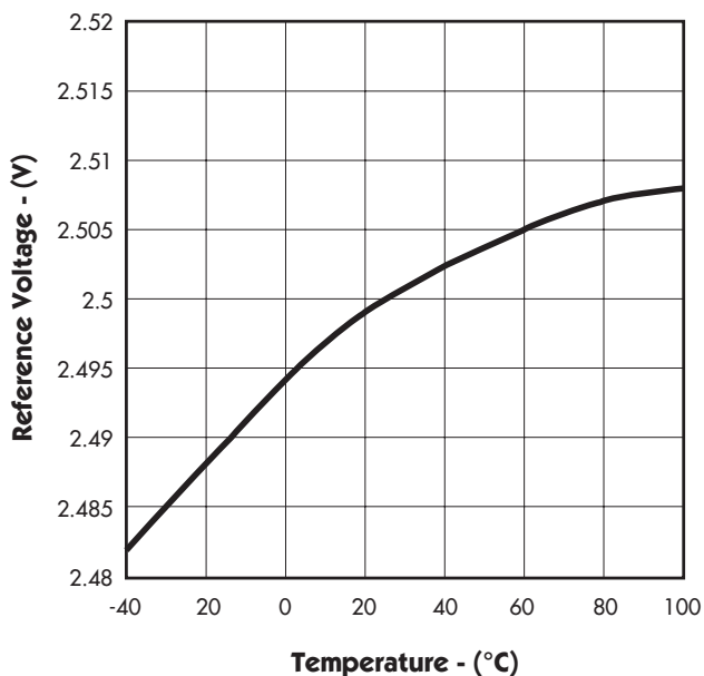
FIGURE 11. — TEMPERATURE DRIFT
