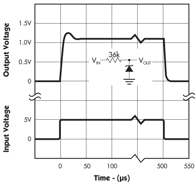
FIGURE 7. — RESPONSE TIME
