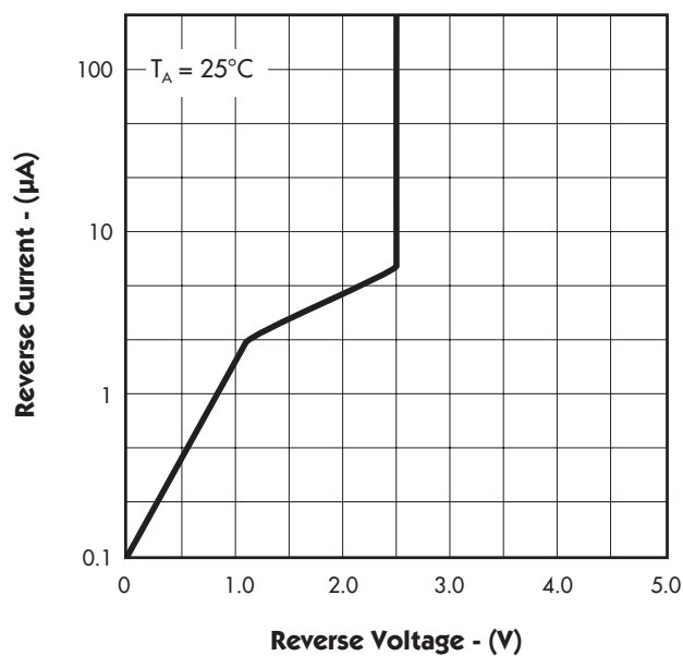
FIGURE 9. — REVERSE CHARACTERISTICS
