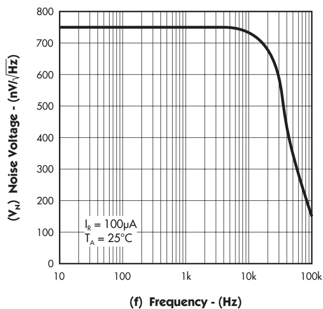
FIGURE 6. — NOISE VOLTAGE
