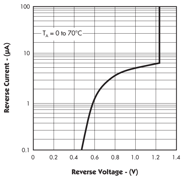
FIGURE 2. — REVERSE CHARACTERISTICS
