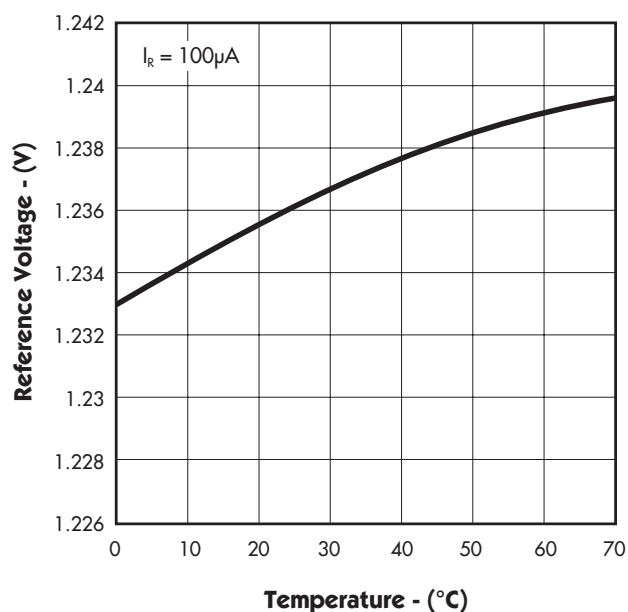
FIGURE 1. — TEMPERATURE DRIFT
