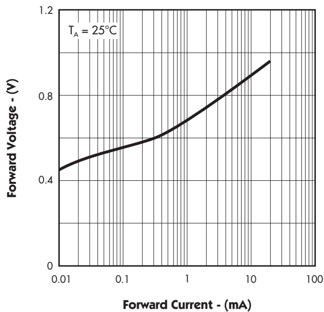
FIGURE 4. — FORWARD CHARACTERISTICS
