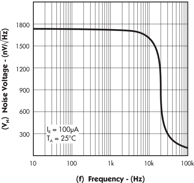
FIGURE 12. — NOISE VOLTAGE
