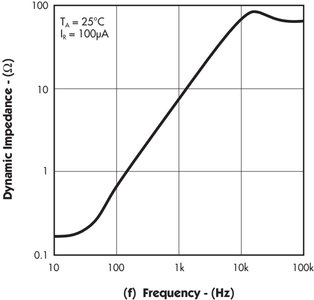
FIGURE 13. — REVERSE DYNAMIC IMPEDANCE
