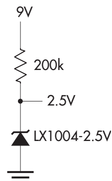
MICROPOWER REFERENCE FROM 9V BATTERY
