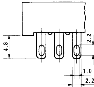
(2) Eyelet (E)
