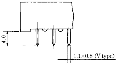
(1) Through hole
