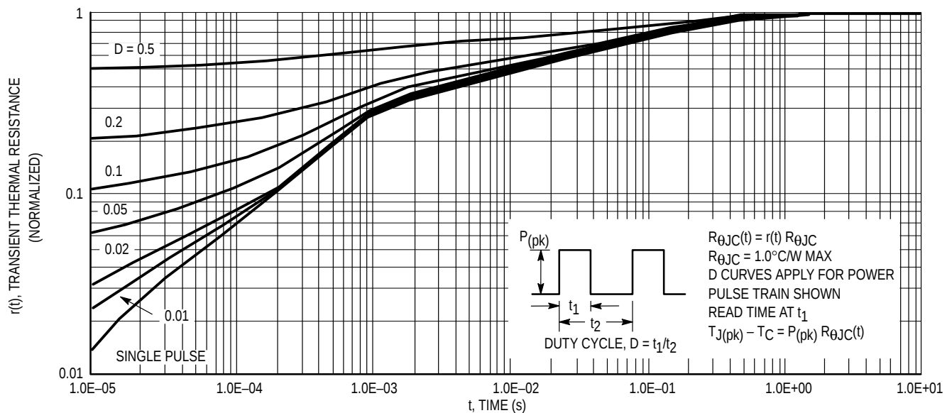
Figure 14. Thermal Response
