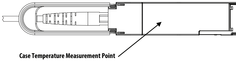
Figure 7. Case Temperature Measurement Point
