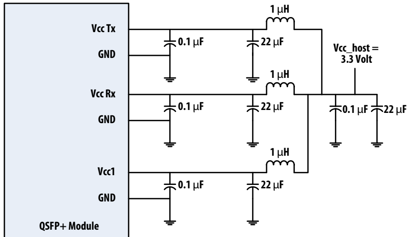
Figure 8. Recommended Host Board Power Supply Filter
