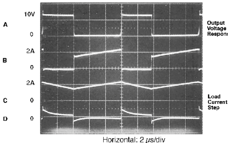
Figure 47. Switching Waveforms
