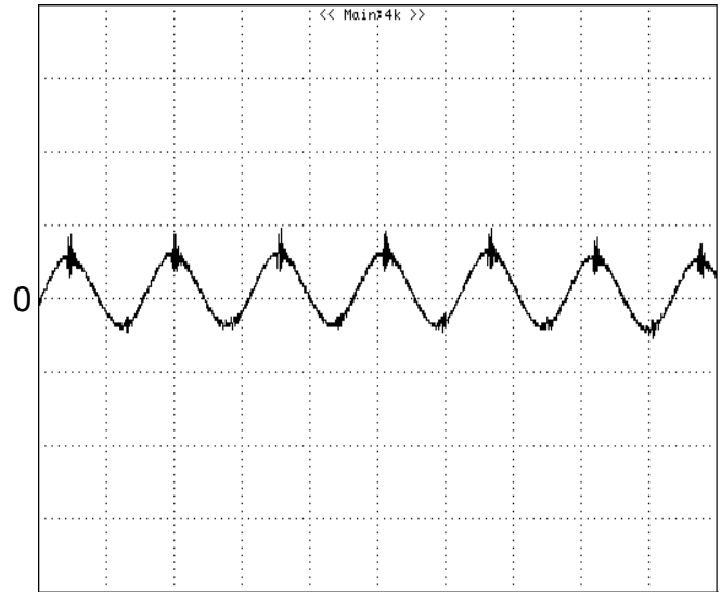
Figure 12: Input reflected ripple current, i_s , through a 12\mu\text{H} source inductor at nominal input voltage and rated load current (20 mA/div, 2 μs/div).
