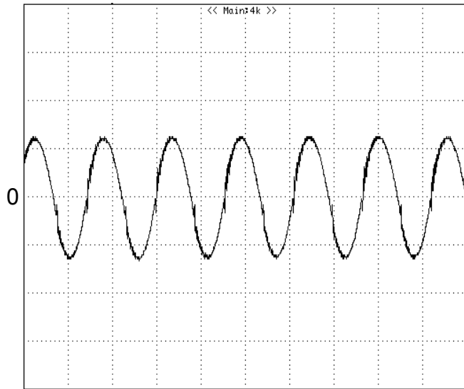
Figure 11: Input Terminal Ripple Current, i_c , at full rated output current and nominal input voltage with 12\mu\text{H} source impedance and 33\mu\text{F} electrolytic capacitor (500 mA/div, 2 μs/div).
