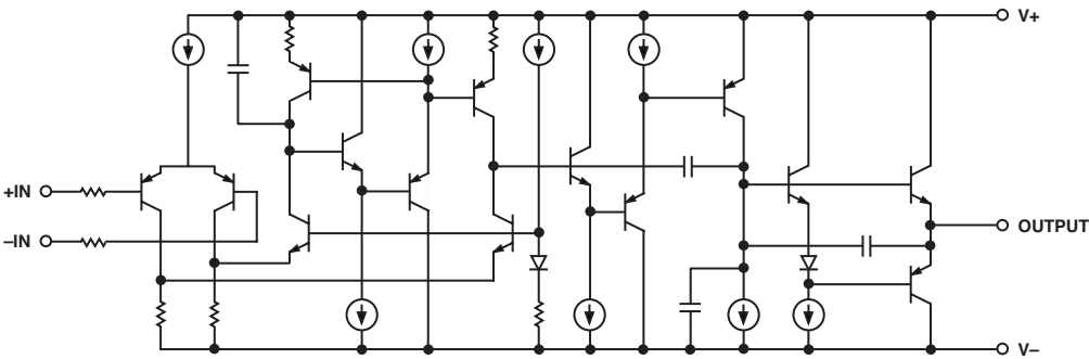
Figure 1. Simplified Schematic
