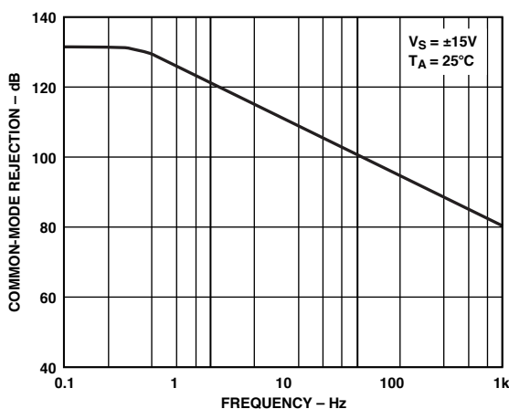
TPC 11. Common-Mode Rejection vs. Frequency
