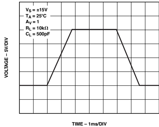
TPC 15. Large-Signal Transient Response
