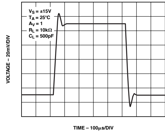
TPC 14. Small-Signal Transient Response
