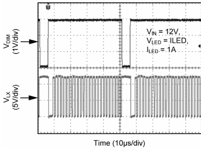
20kHz Dimming @ 90% Duty
