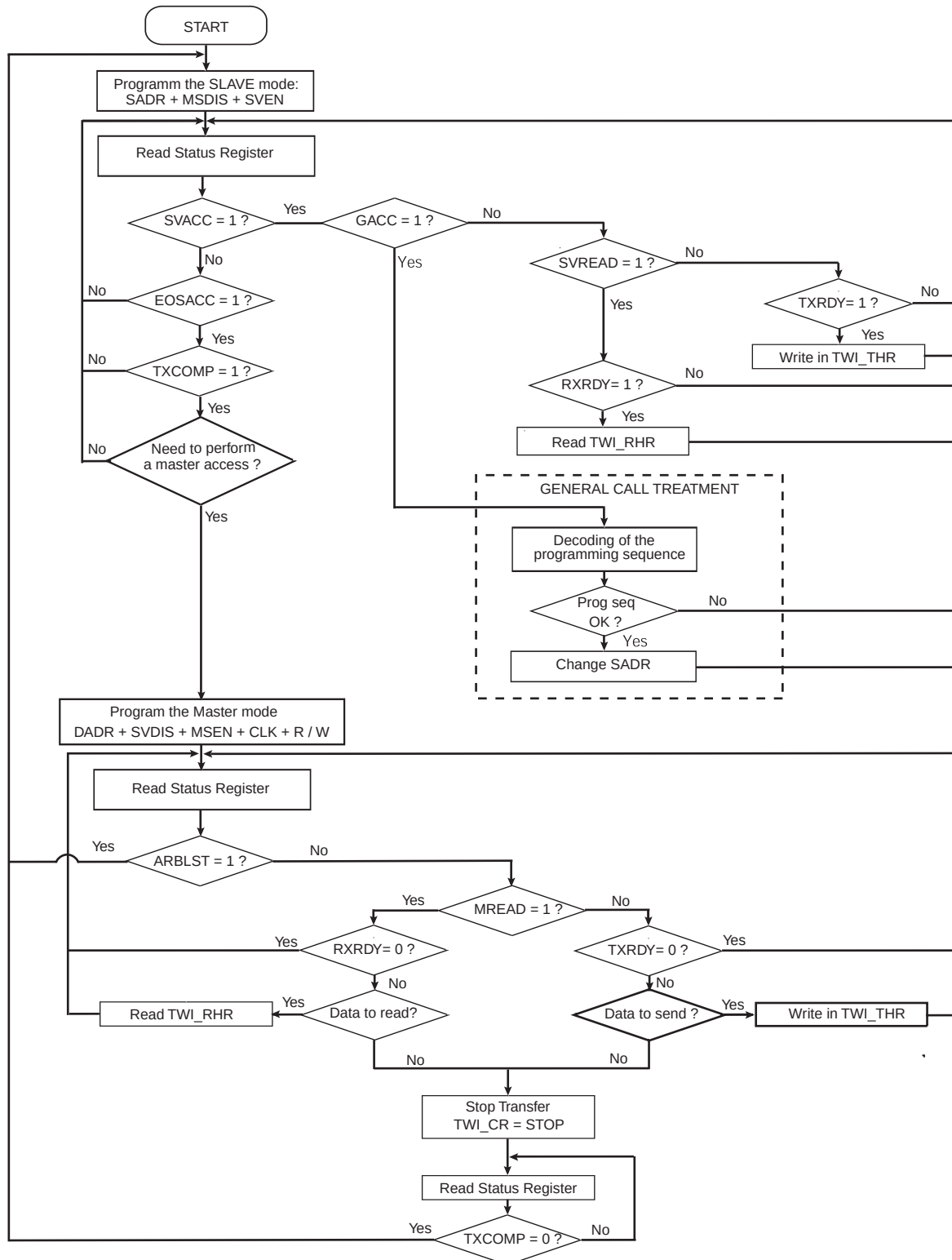
Figure 30-23. Multi-master Flowchart
