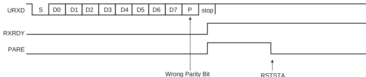
Figure 31-7. Parity Error
