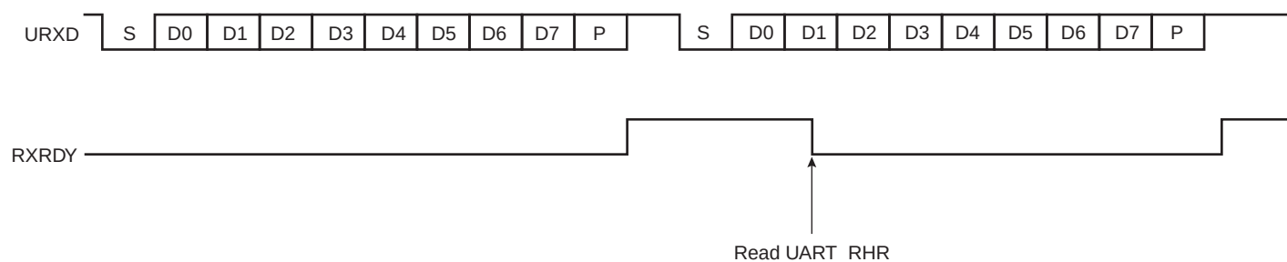
Figure 31-5. Receiver Ready
