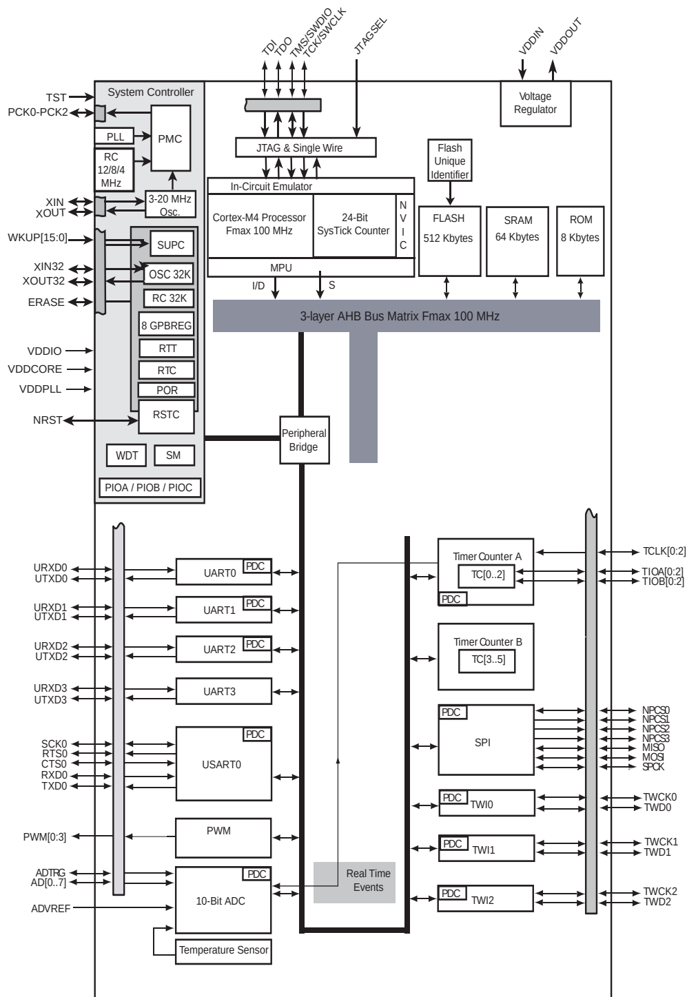
Figure 2-3. SAM4N8 48-pin Version Block Diagram
