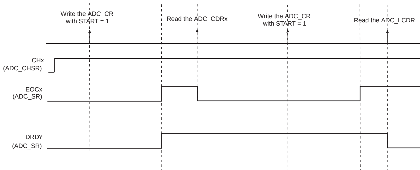
Figure 35-3. EOCx and DRDY Flag Behavior
