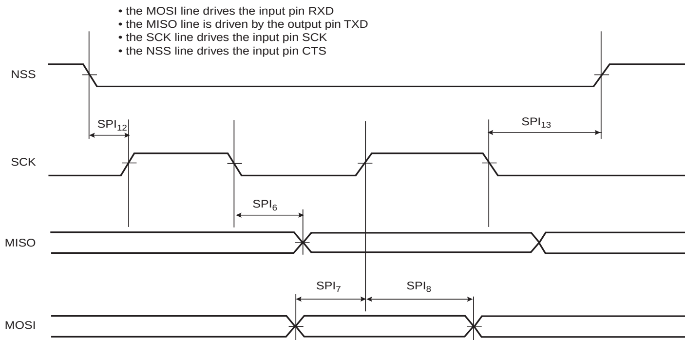
Figure 37-17. Two-wire Serial Bus Timing
