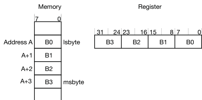
Figure 13-6. Little-endian Format
