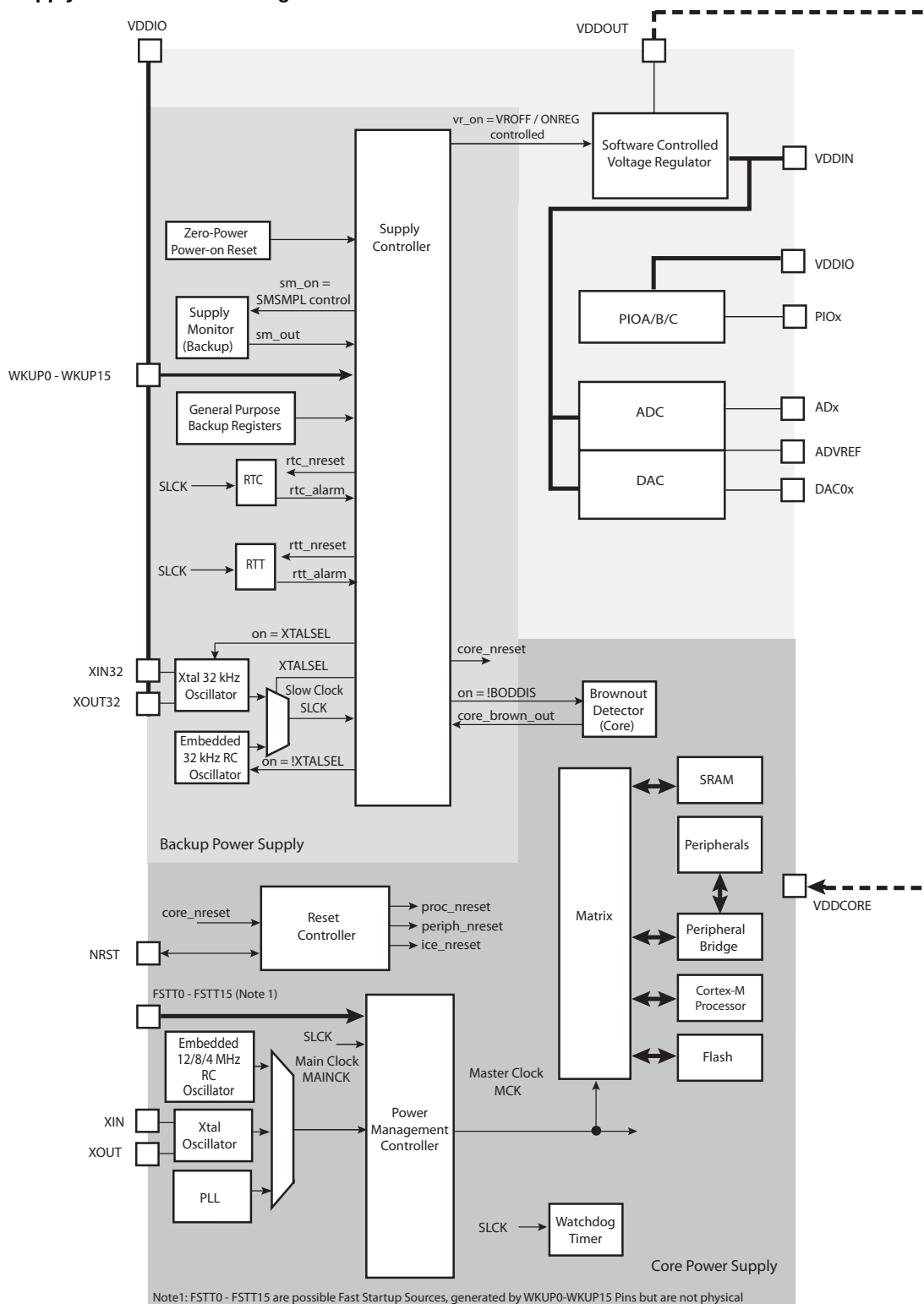
Figure 19-1. Supply Controller Block Diagram
