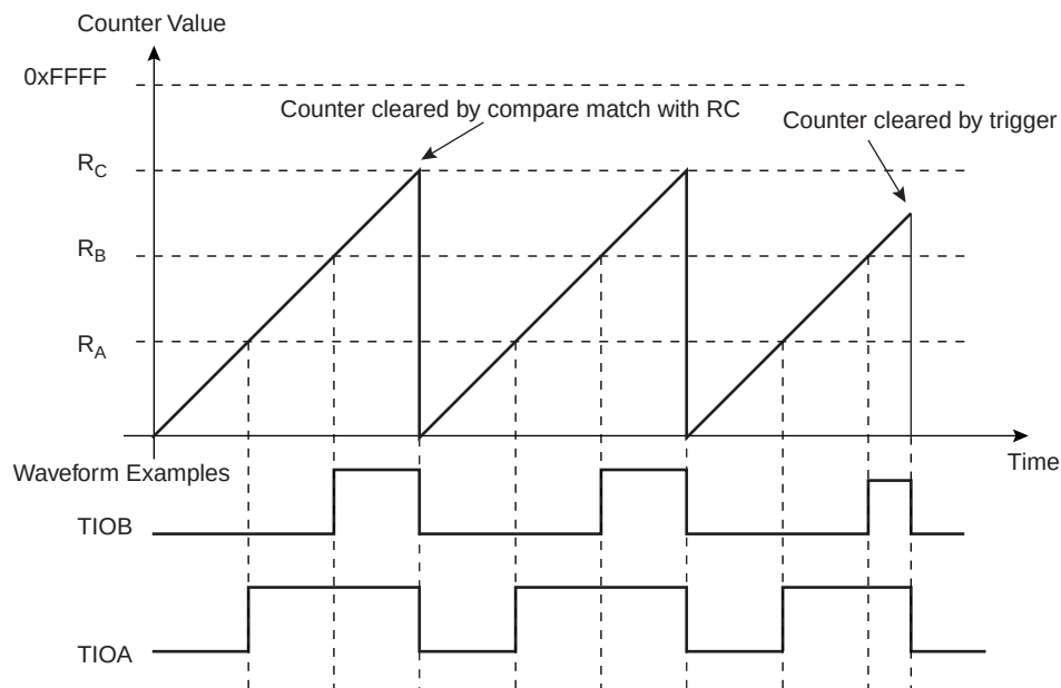
Figure 33-12. WAVSEL = 10 With Trigger
