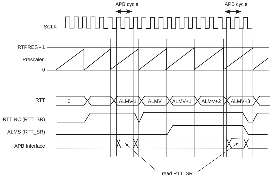
Figure 16-2. RTT Counting
