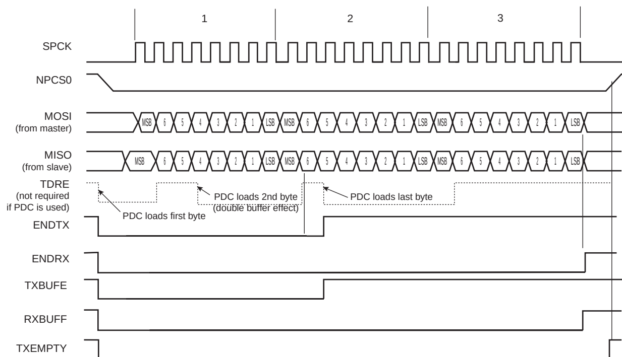
Figure 29-8. PDC Status Register Flags Behavior
