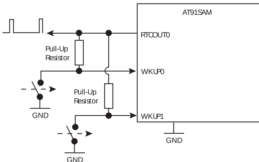
Figure 19-5. Low Power Debouncer (Push-to-Make switch, pull-up resistors)
