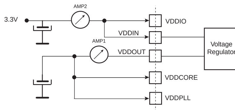
Figure 37-7. Measurement Setup for Wait Mode
