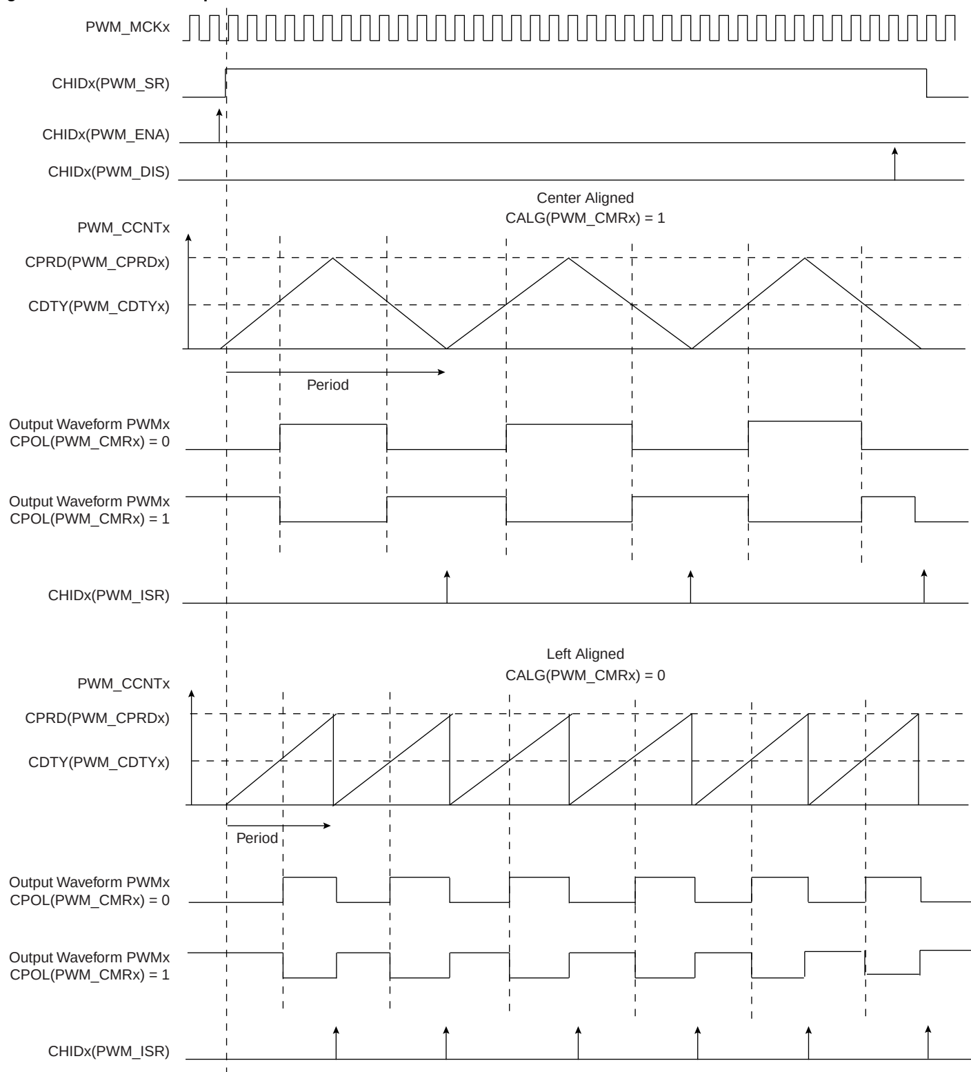
Figure 34-5. Waveform Properties
