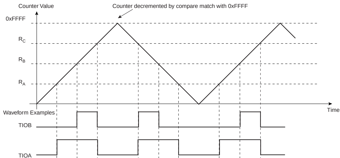
Figure 33-13. WAVSEL = 01 Without Trigger
