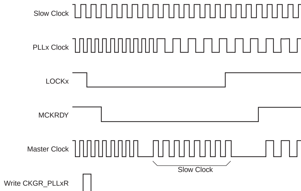
Figure 26-10. Change PLLx Programming
