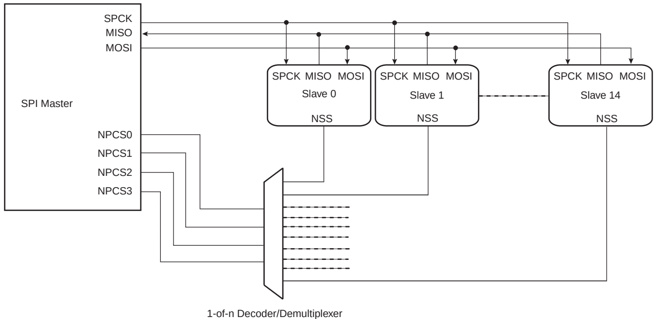
Figure 29-10. Chip Select Decoding Application Block Diagram: Single Master/Multiple Slave Implementation
