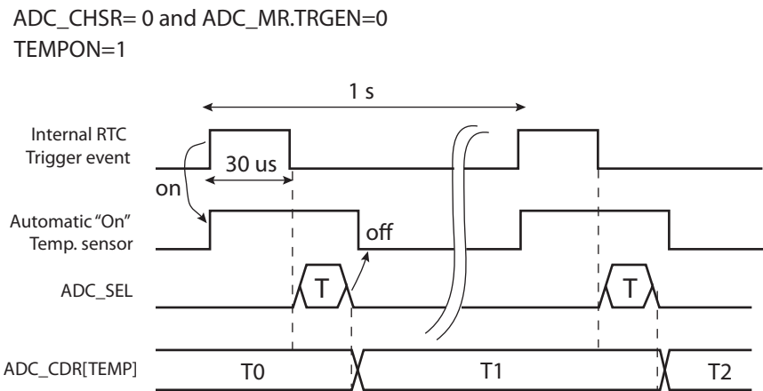
Figure 35-8. Temperature Conversion Only
