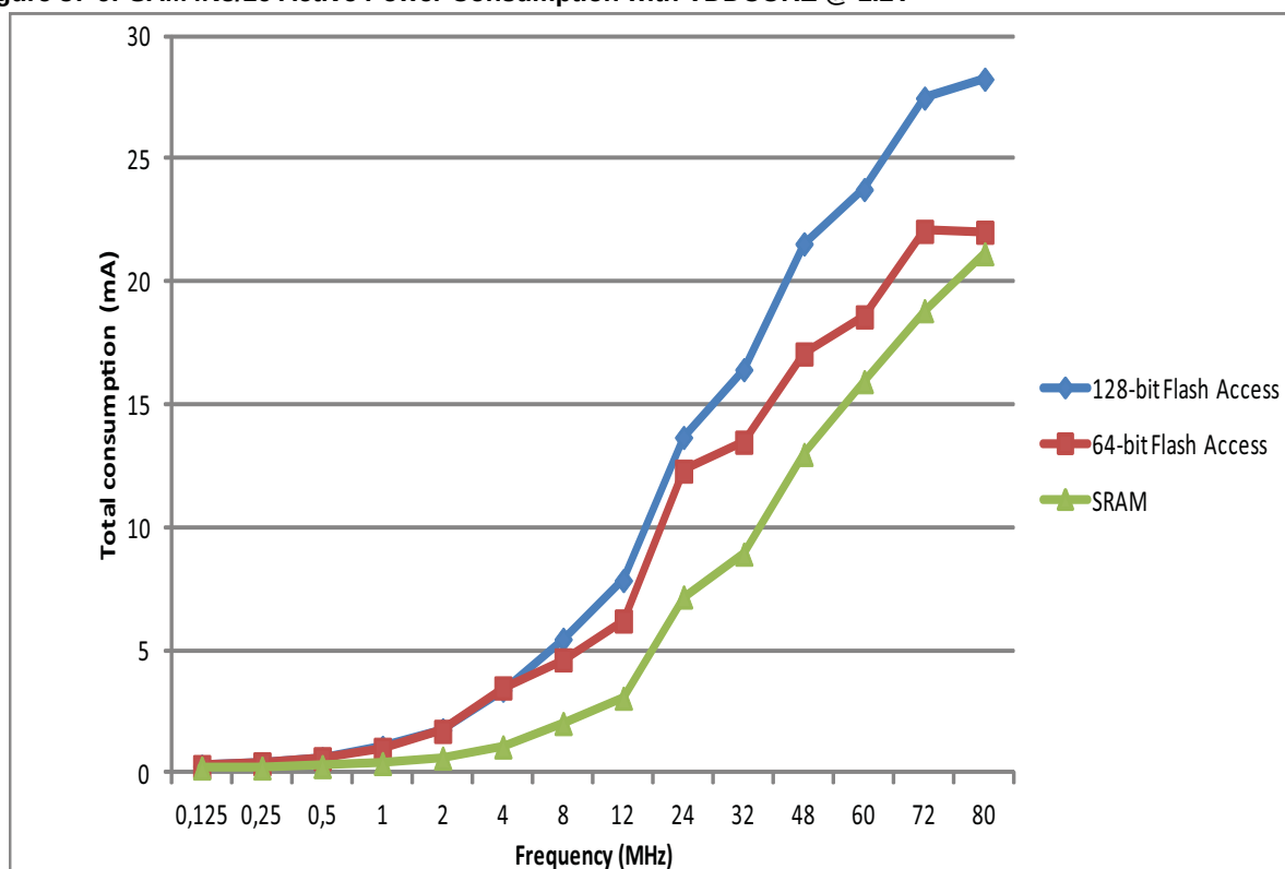
Figure 37-9. SAM4N8/16 Active Power Consumption with VDDCORE @ 1.2V
