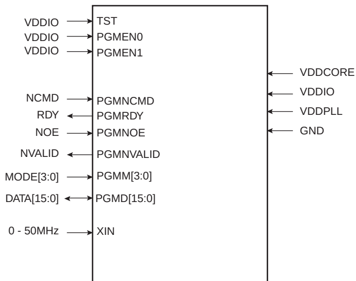
Figure 22-1. SAM4Nx8/C Parallel Programming Interface
