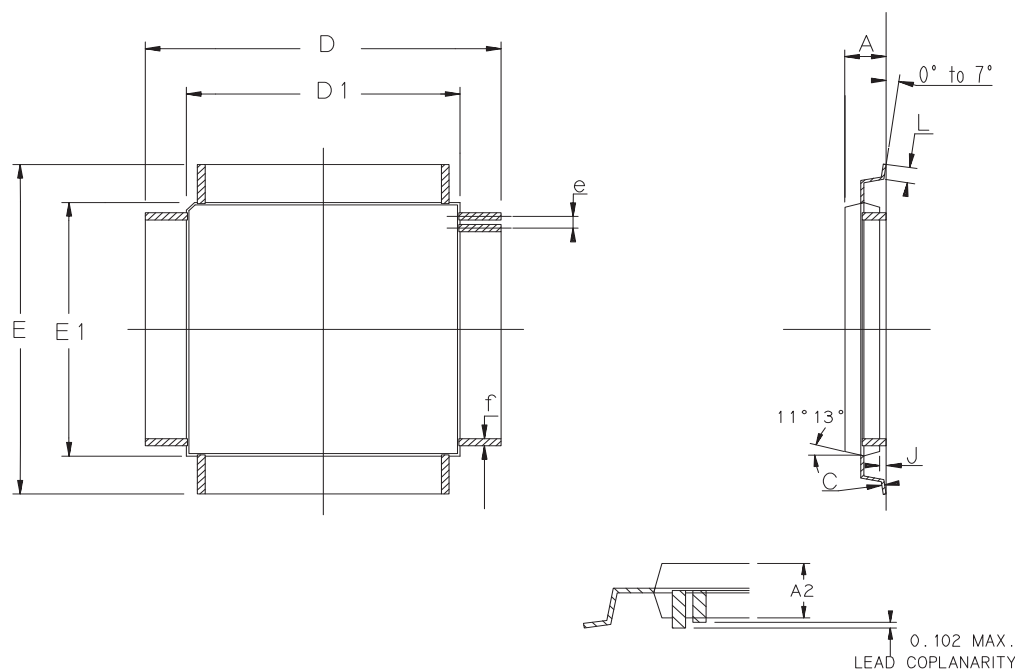
Figure 38-6. 48-lead LQFP Package Drawing
