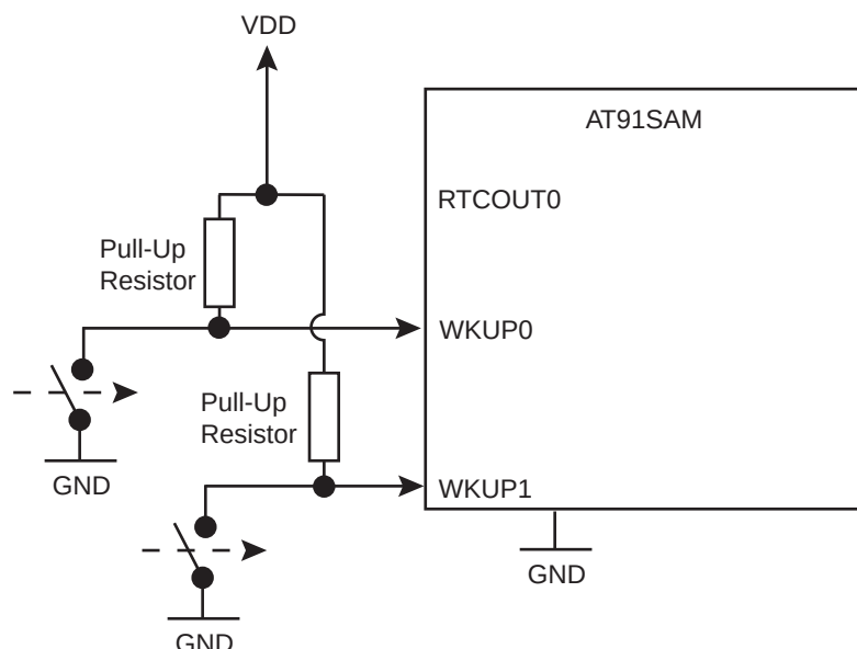
Figure 19-7. Using WKUP0/WKUP1 without RTCOUT Pins
