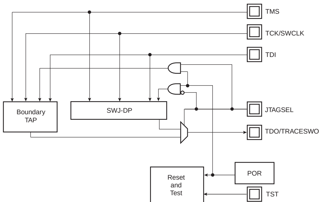
Figure 14-1. Debug and Test Block Diagram
