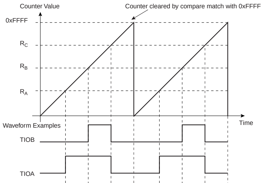
Figure 33-9. WAVSEL= 00 without trigger
