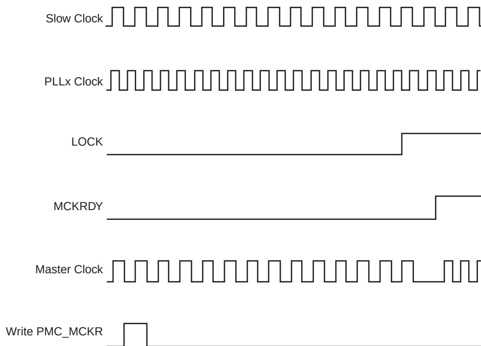
Figure 26-8. Switch Master Clock from Slow Clock to PLLx Clock
