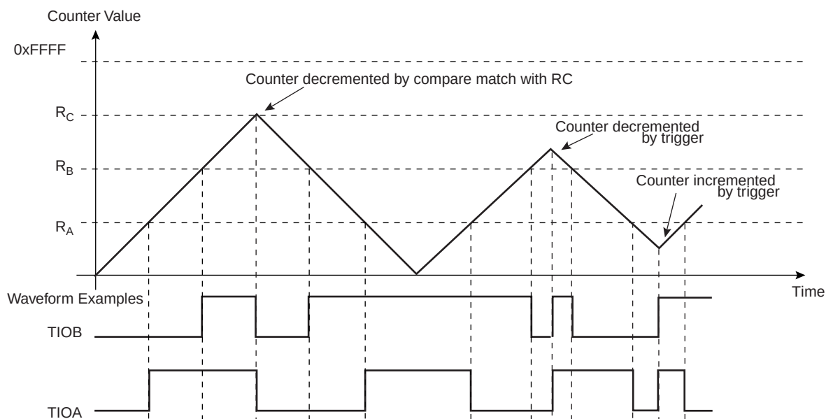
Figure 33-16. WAVSEL = 11 With Trigger
