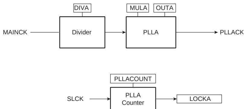
Figure 26-4. Divider and PLL Block Diagram
