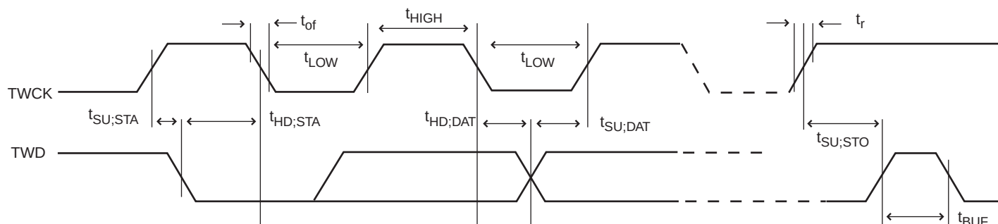
Figure 37-16.USART SPI Slave Mode (Mode 1 or 2)
