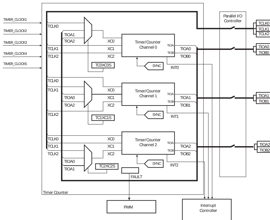
Figure 33-2. Timer Counter Block Diagram
