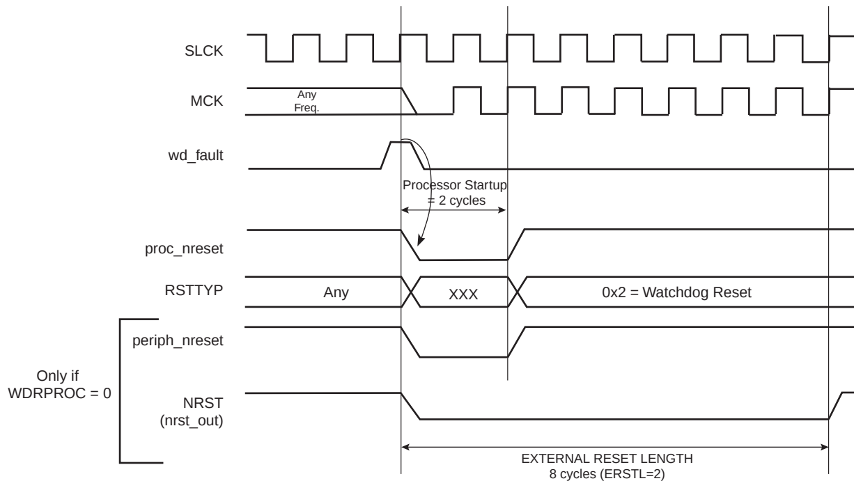
Figure 15-6. Watchdog Reset
