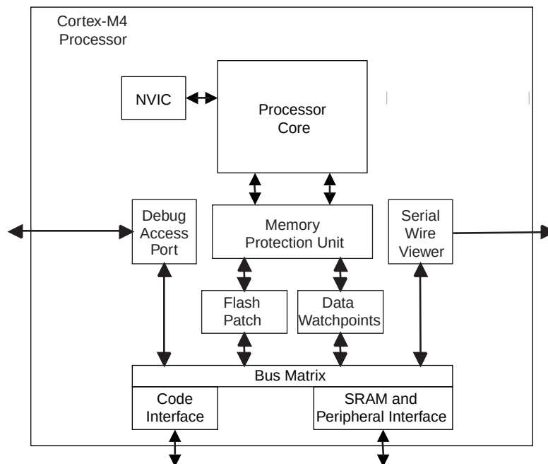
Figure 13-1. Typical Cortex-M4 Implementation
