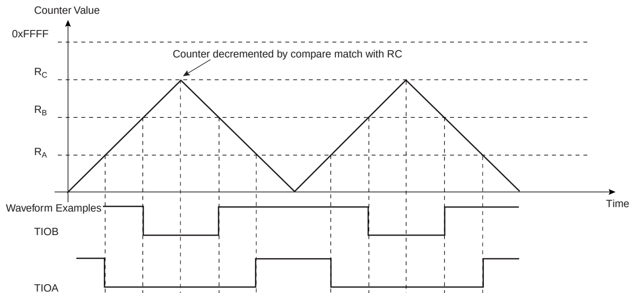
Figure 33-15. WAVSEL = 11 Without Trigger
