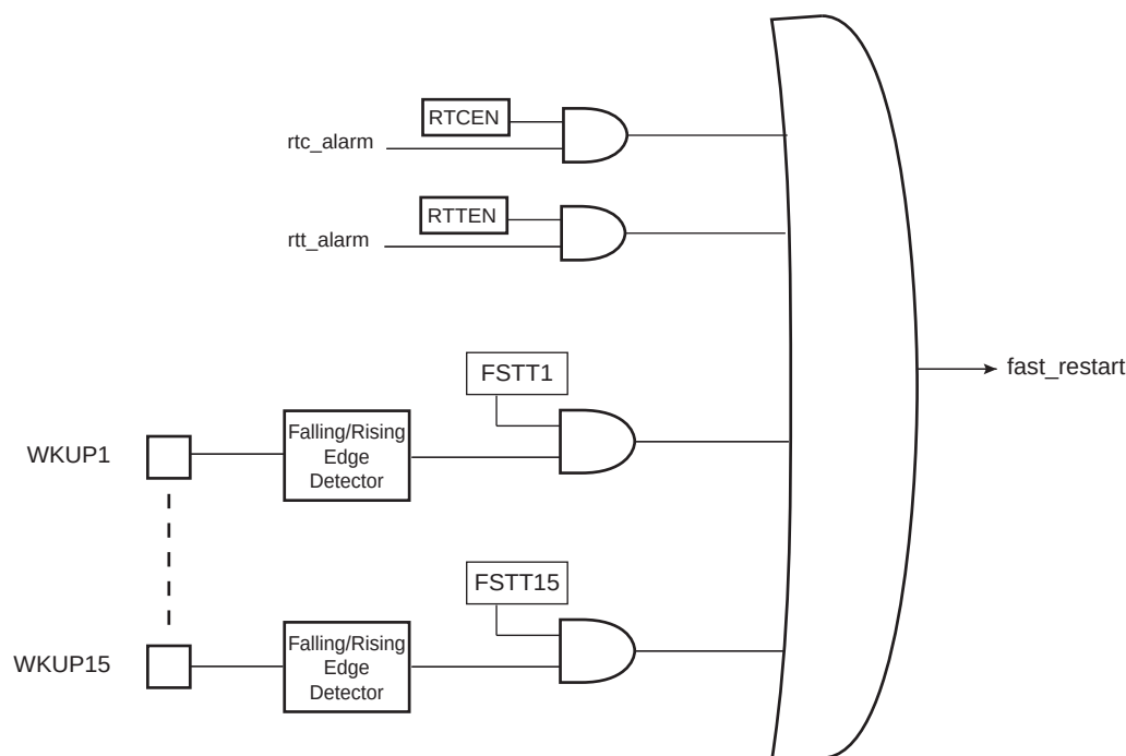
Figure 5-5. Fast Start-up Source
