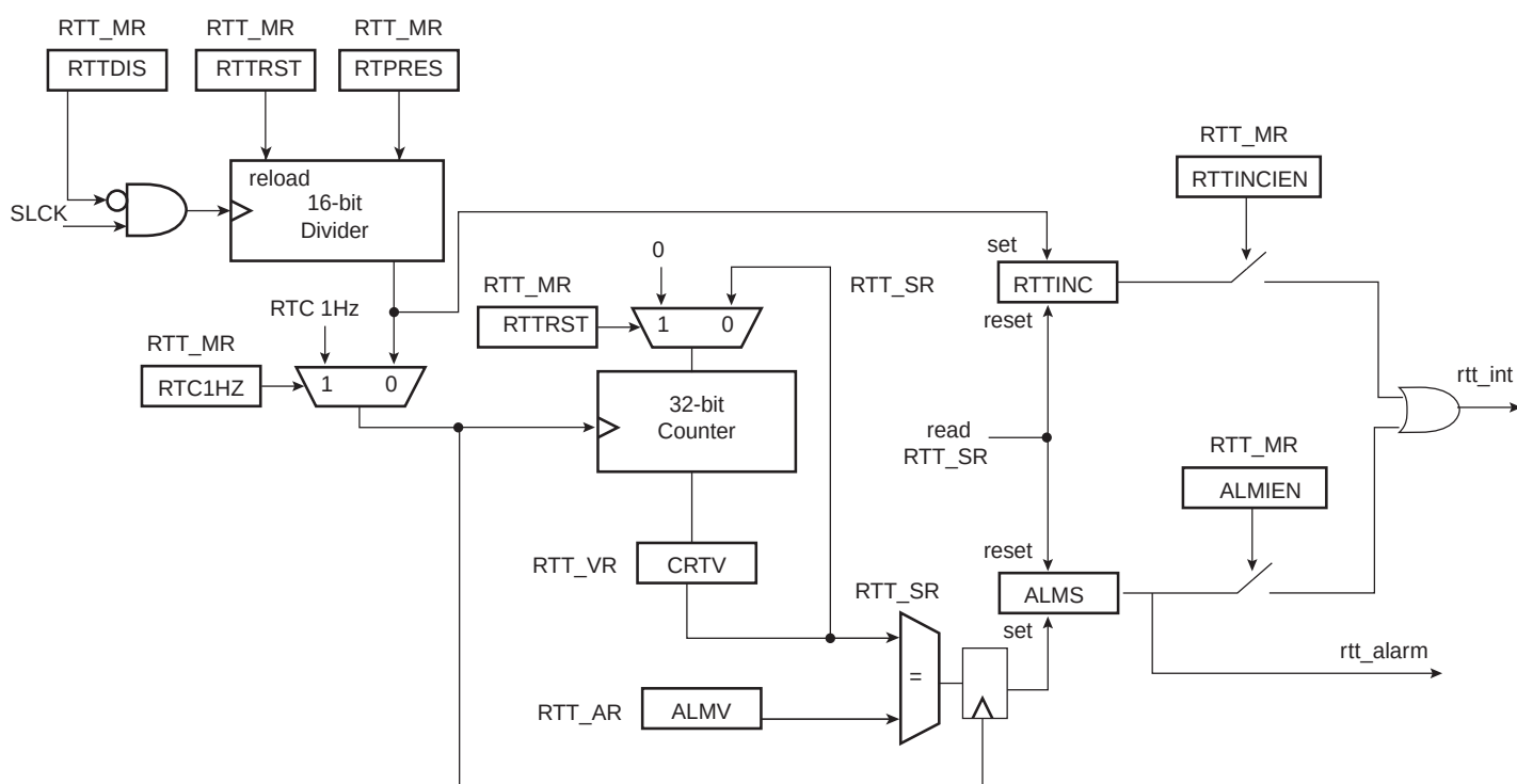
Figure 16-1. Real-time Timer
