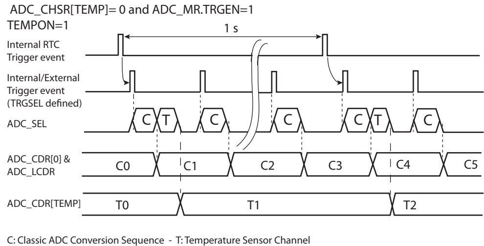
Figure 35-7. Optimized Temperature Conversion combined with classical conversions
