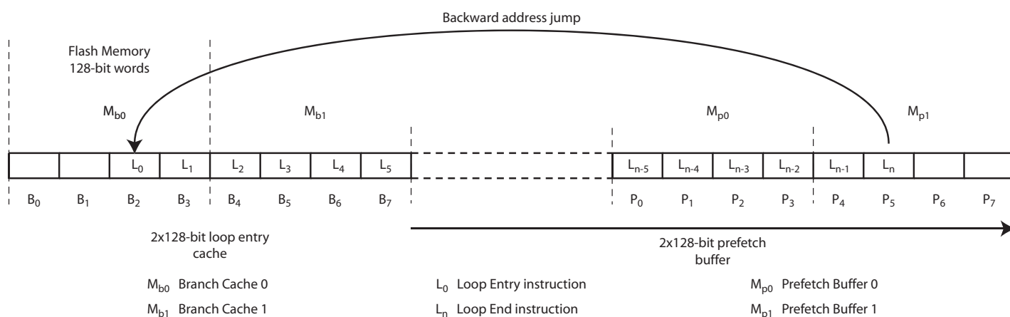
Figure 21-4. Code Loops Optimization
