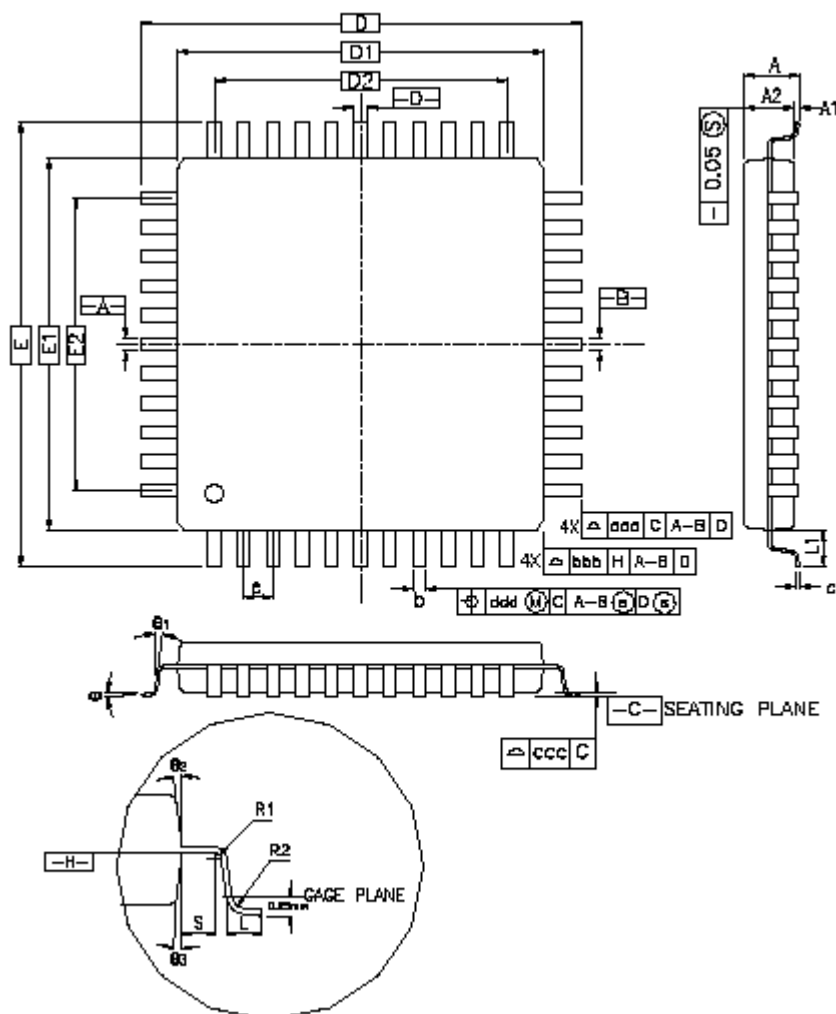
Figure 38-4. 64-lead LQFP Package Drawing
