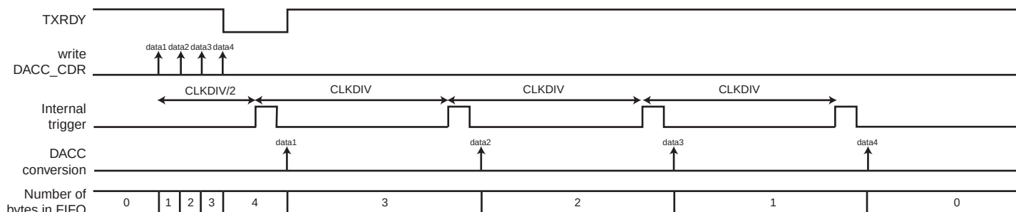
Figure 36-2. Internal trigger
