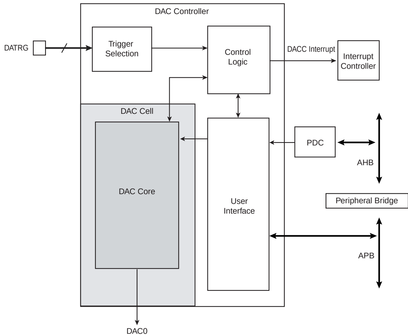
Figure 36-1. Digital-to-Analog Converter Controller Block Diagram
