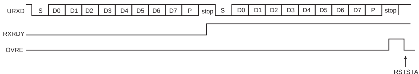
Figure 31-6. Receiver Overrun
