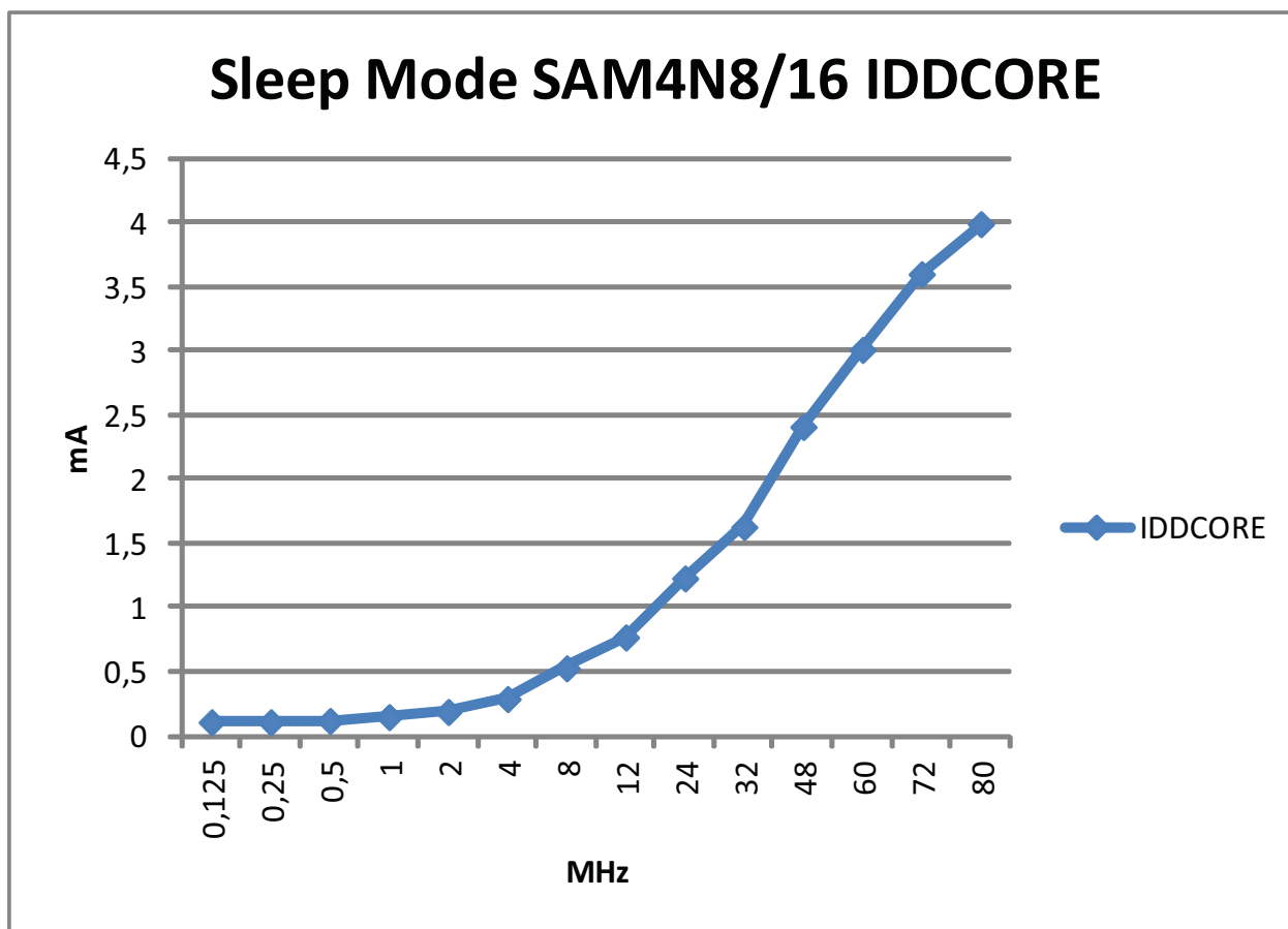
Figure 37-6. Current Consumption in Sleep Mode (AMP1) versus Master Clock Ranges (Condition from Table 37-11 and Table 37-12)
