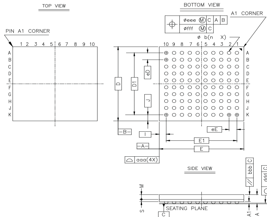
Figure 38-3. 100-ball VFBGA Package Drawing
