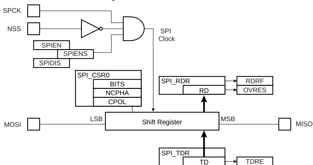
Figure 29-12. Slave Mode Functional Block Diagram
