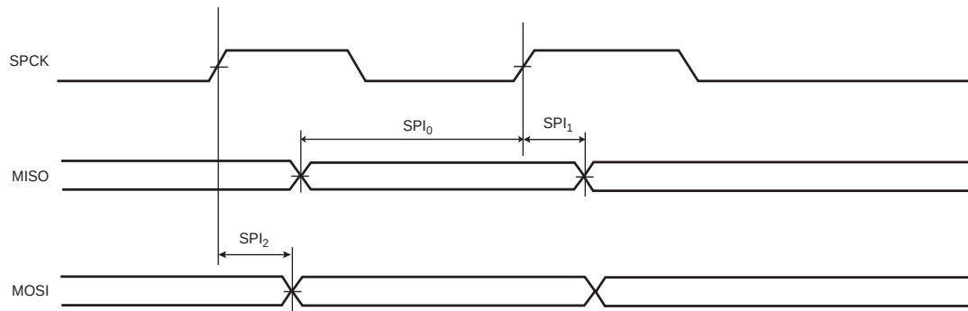
Figure 37-11. SPI Master Mode with (CPOL = NCPHA = 0) or (CPOL = NCPHA = 1)
