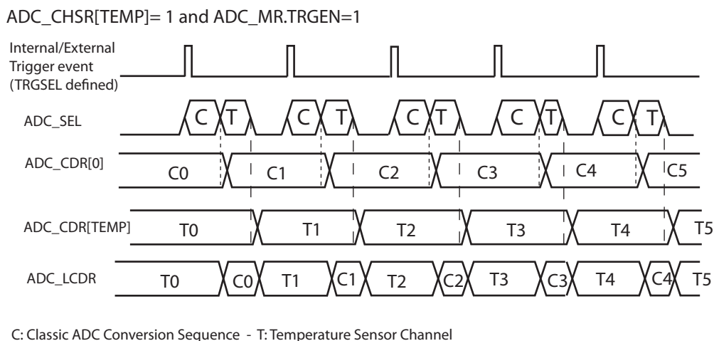
Figure 35-6. Non-optimized Temperature Conversion
