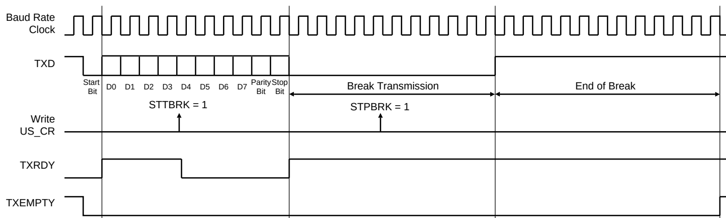
Figure 32-16. Break Transmission
