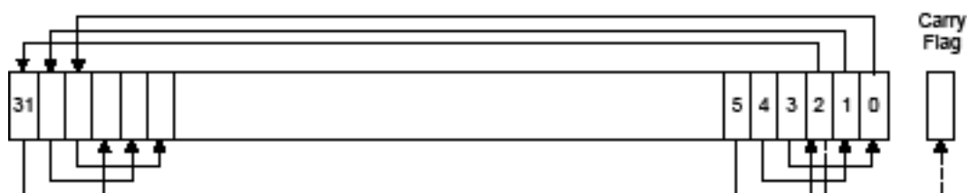
Figure 13-12.ROR #3
