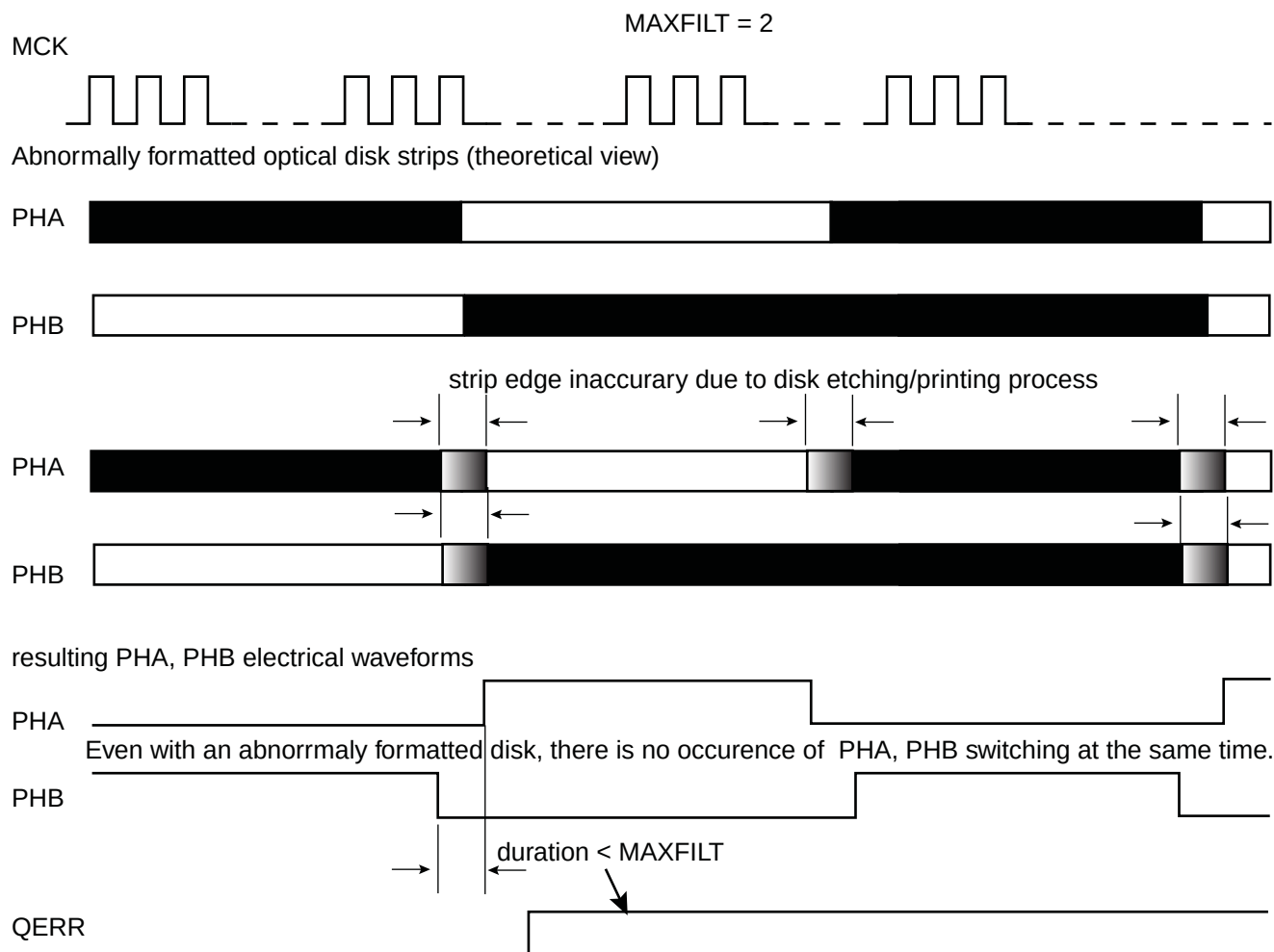
Figure 33-21. Quadrature Error Detection
