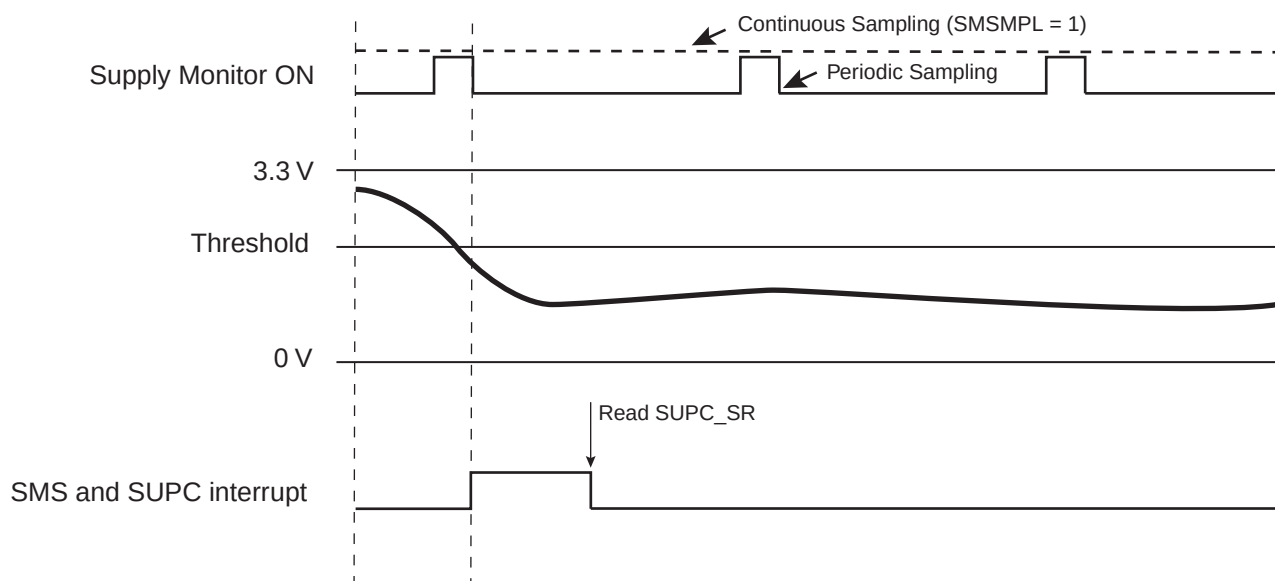
Figure 19-2. Supply Monitor Status Bit and Associated Interrupt
