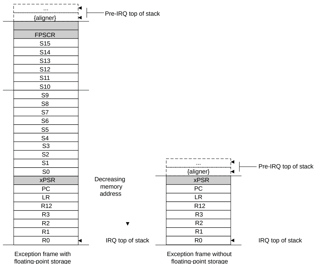
Figure 13-8. Exception Stack Frame
