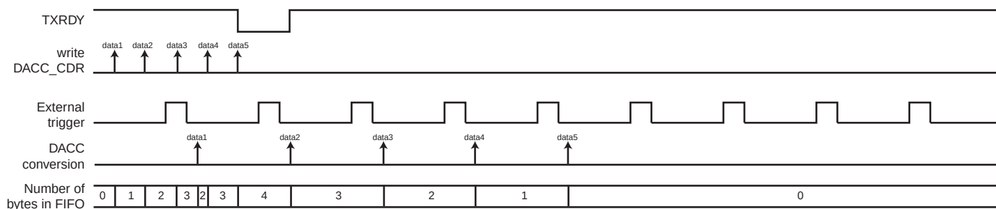
Figure 36-3. External trigger
