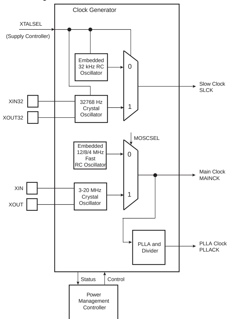
Figure 26-1. Clock Generator Block Diagram
