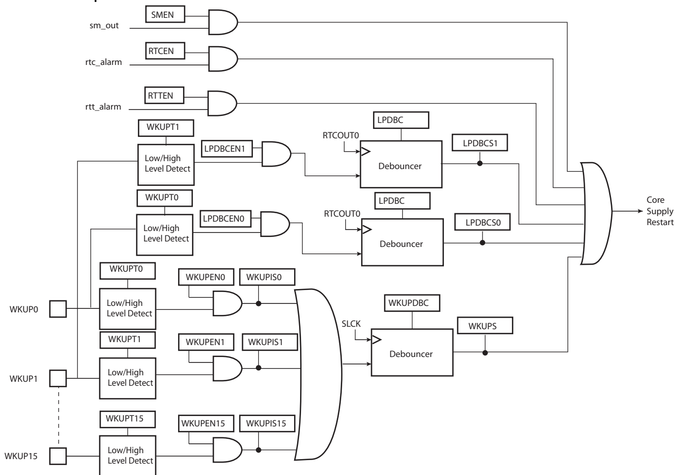
Figure 19-4. Wake-up Sources
