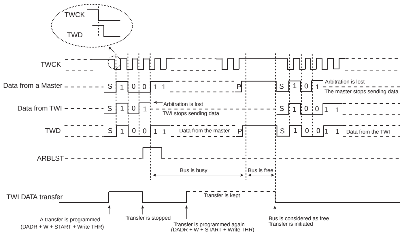
Figure 30-22. Arbitration Cases
