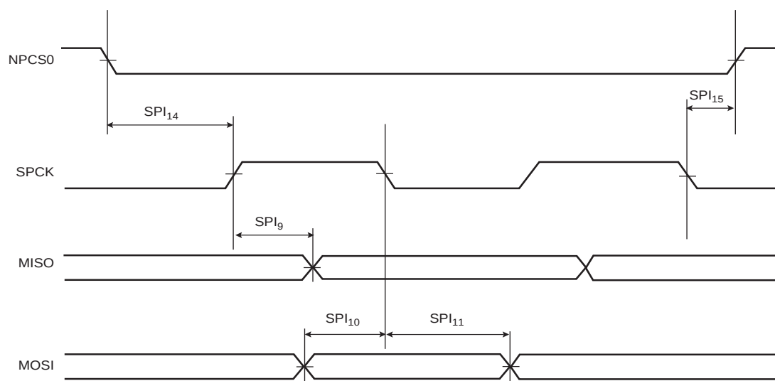
Figure 37-14.SPI Slave Mode with(CPOL = NCPHA = 0) or (CPOL = NCPHA = 1)
