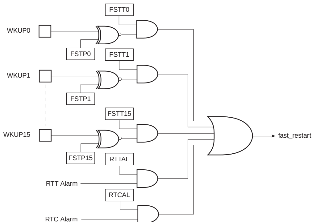
Figure 26-7. Fast Start-up Circuitry
