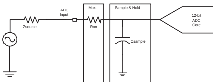
Figure 37-10.Simplified Acquisition Path
