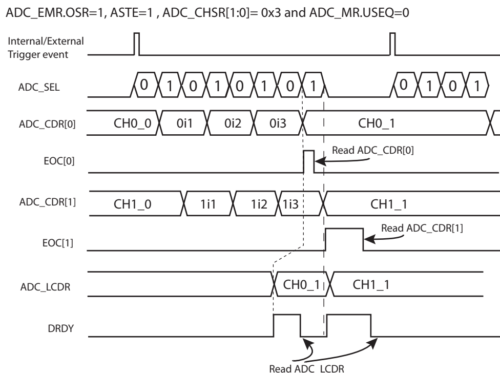
Figure 35-10. Digital Averaging Function Waveforms on a single trigger event
