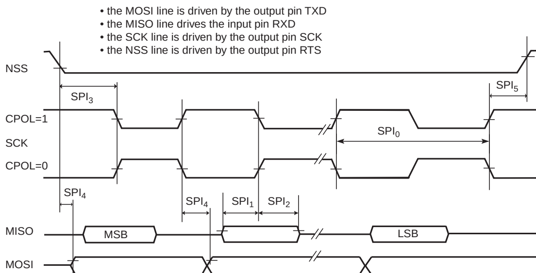
Figure 37-15.USART SPI Master Mode
