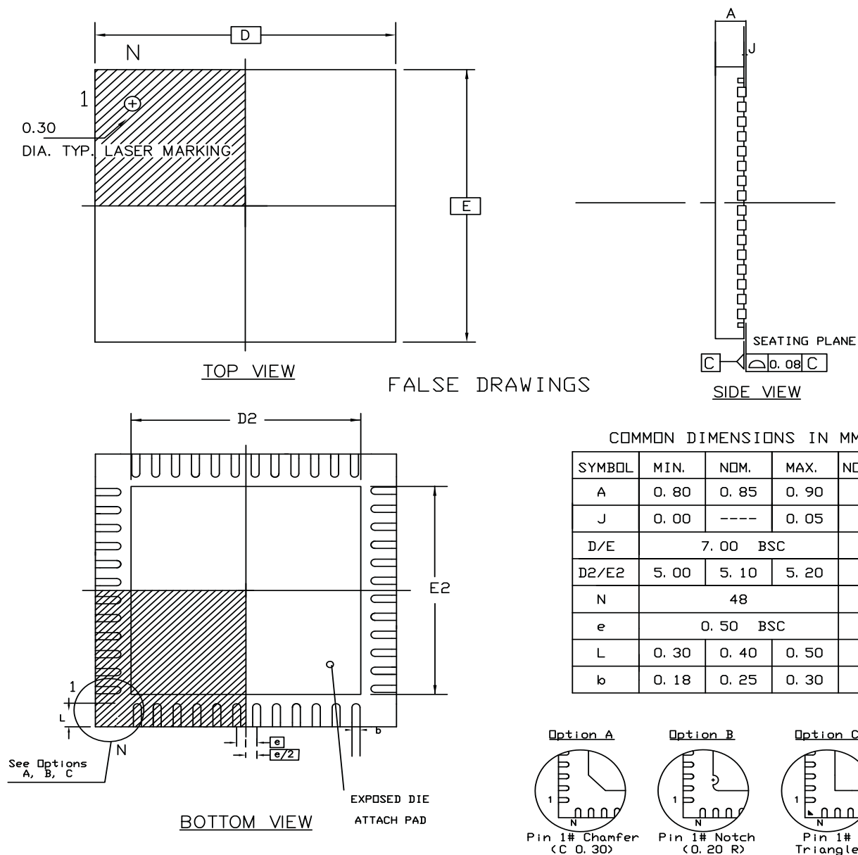
Figure 38-7. 48-pad QFN Package Drawing
