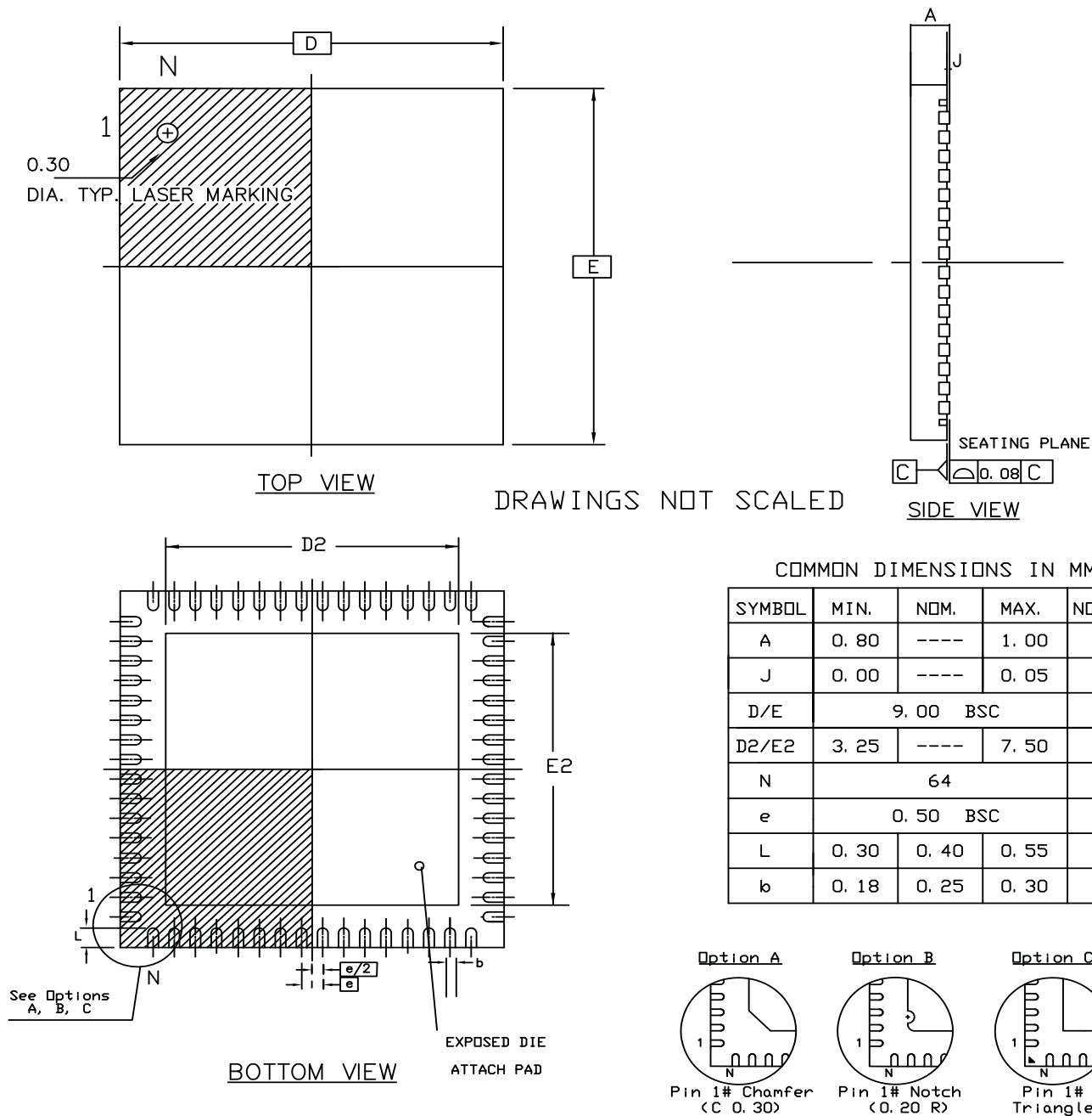
Figure 38-5. 64-pad QFN Package Drawing
