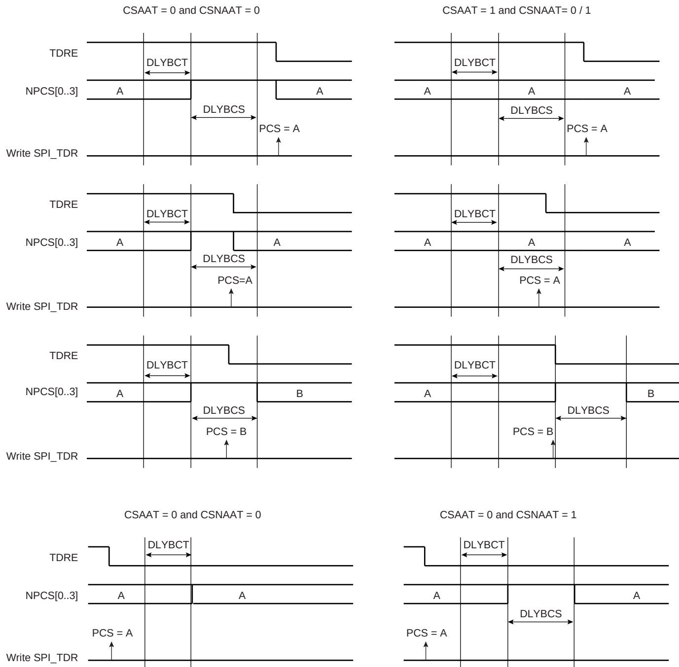
Figure 29-11. Peripheral Deselection
