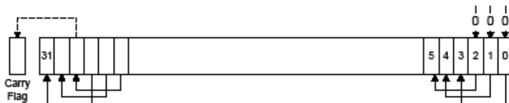
Figure 13-11.LSL #3
