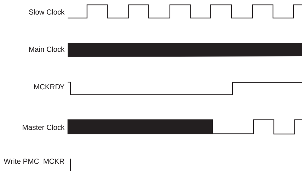
Figure 26-9. Switch Master Clock from Main Clock to Slow Clock
