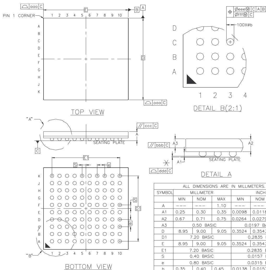
Figure 38-2. 100-ball TFBGA Package Drawing
