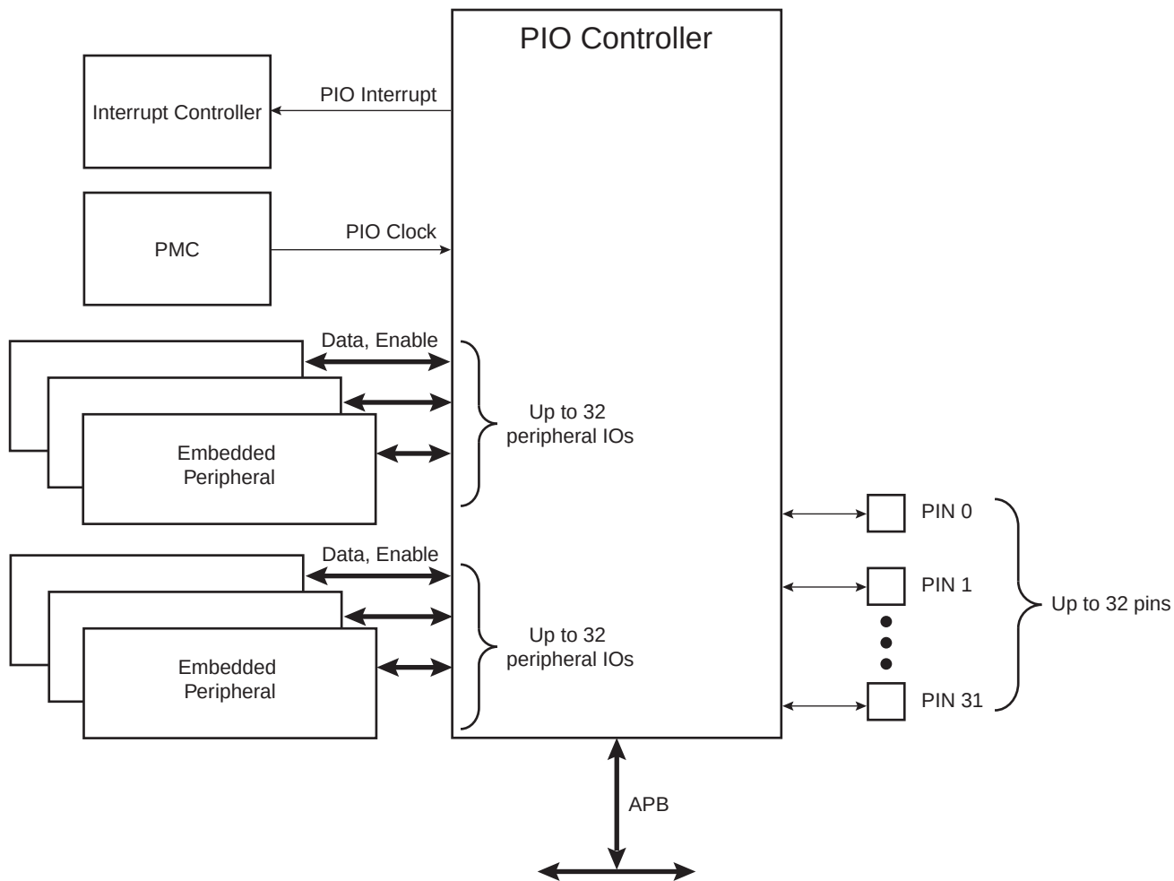
Figure 28-1. Block Diagram
