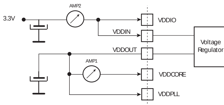
Figure 37-8. Active Mode Measurement Setup
