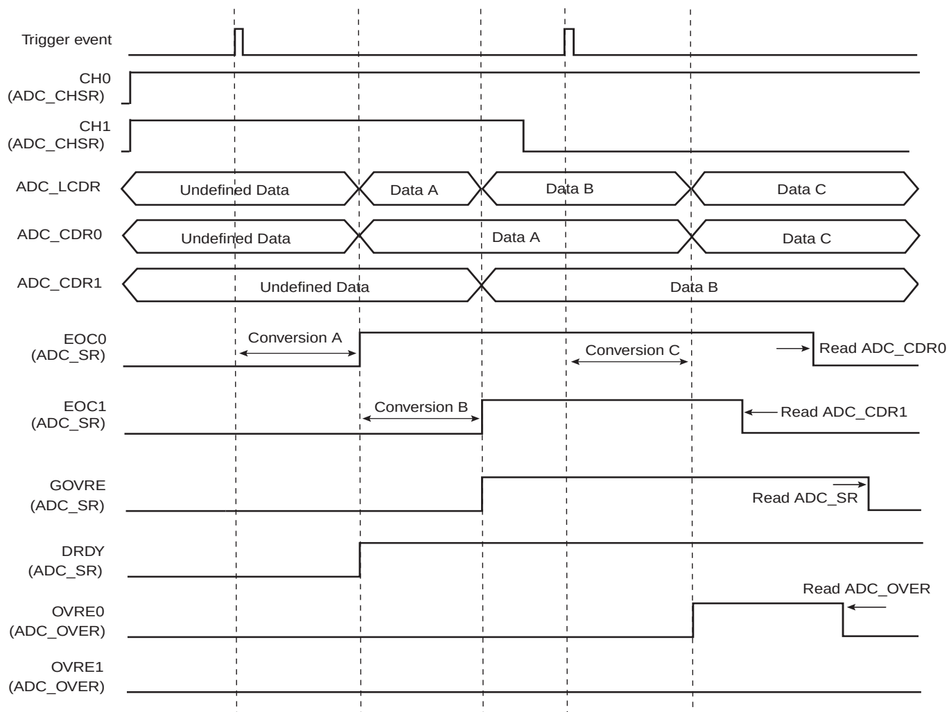
Figure 35-4. GOVRE and OVREx Flag Behavior
