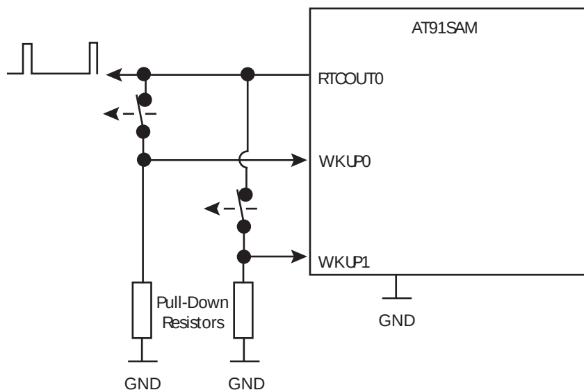
Figure 19-6. Low Power Debouncer (Push-to-Break switch, pull-down resistors)
