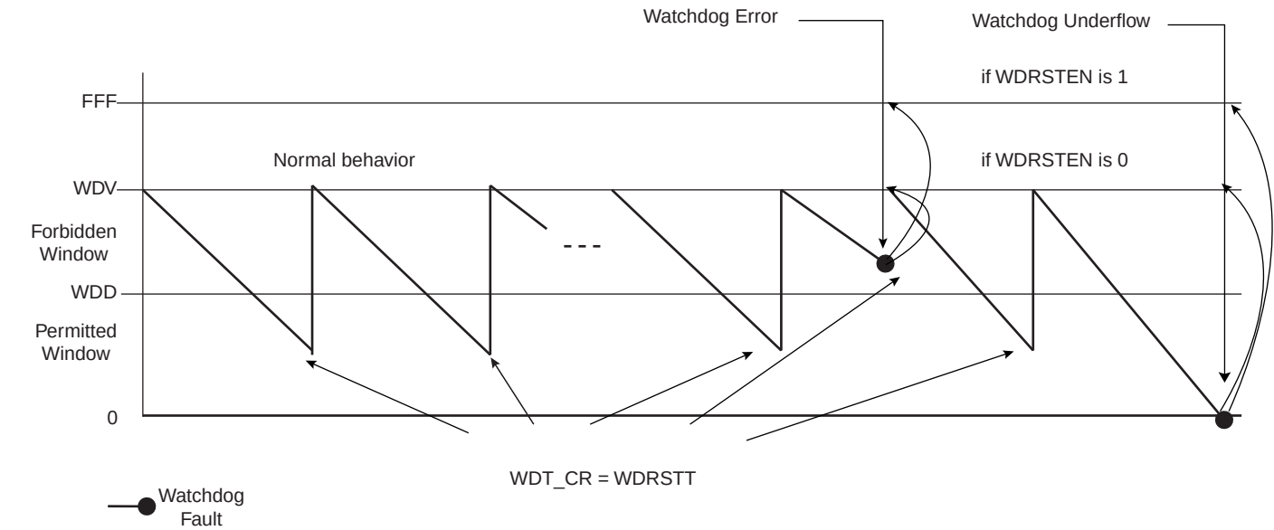
Figure 18-2. Watchdog Behavior
