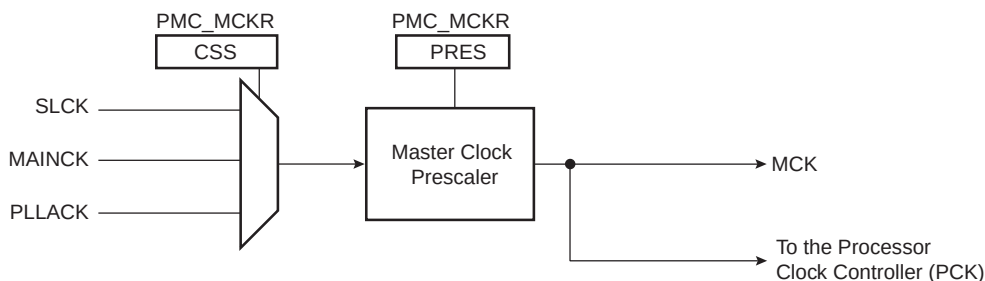
Figure 26-6. Master Clock Controller
