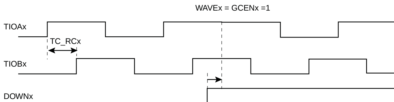
Figure 33-22. 2-bit Gray Up/Down Counter.
