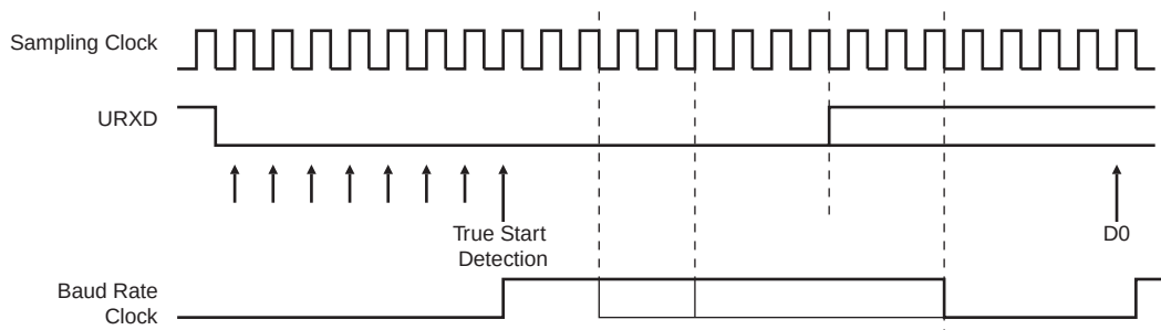
Figure 31-3. Start Bit Detection
