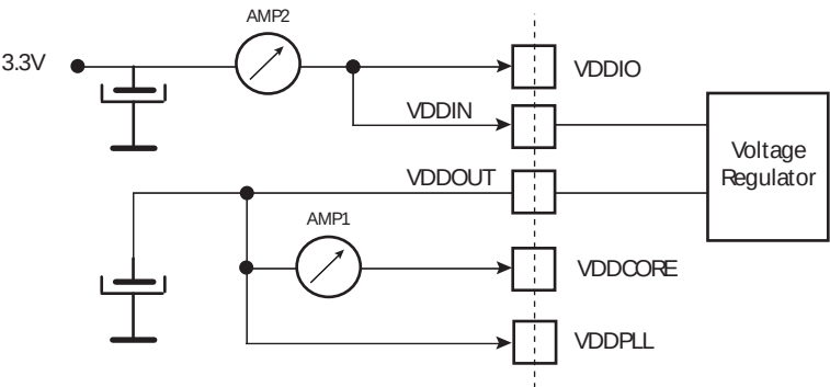
Figure 37-5. Measurement Setup for Sleep Mode
