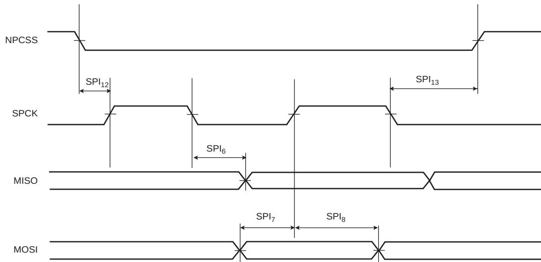
Figure 37-13. SPI Slave Mode with (CPOL = 0 and NCPHA = 1) or (CPOL = 1 and NCPHA = 0)
