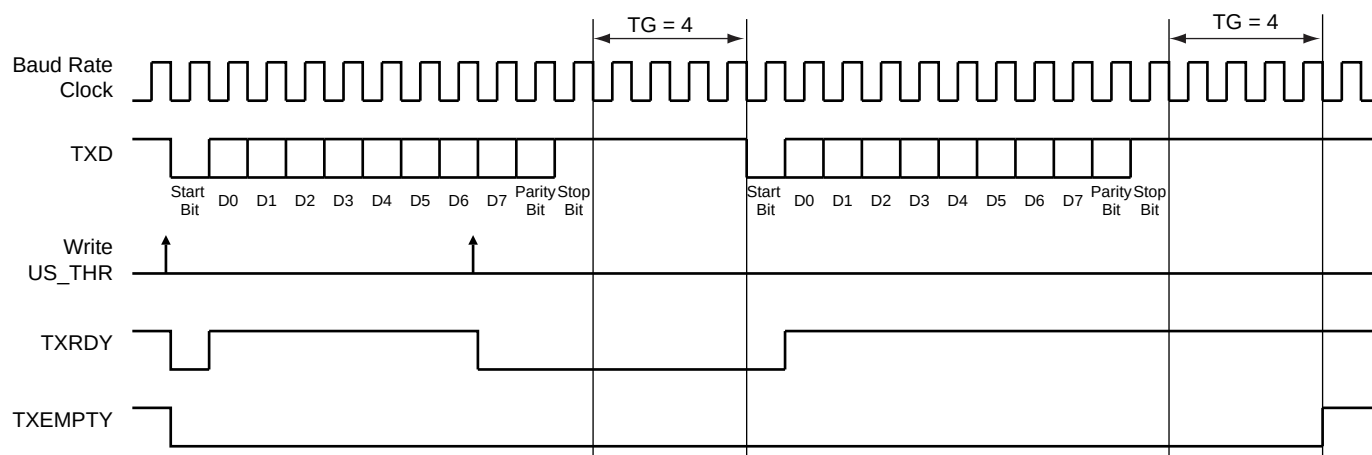
Figure 32-13. Timeguard Operations
