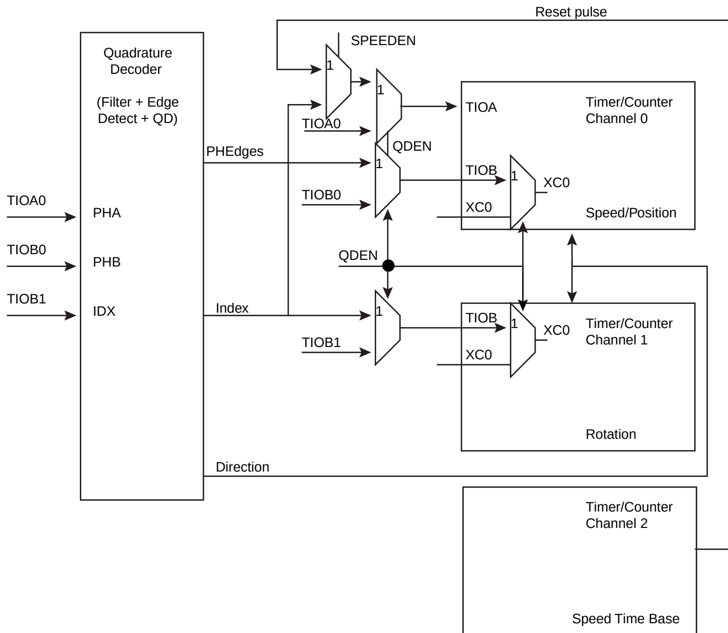
Figure 33-17. Predefined Connection of the Quadrature Decoder with Timer Counters
