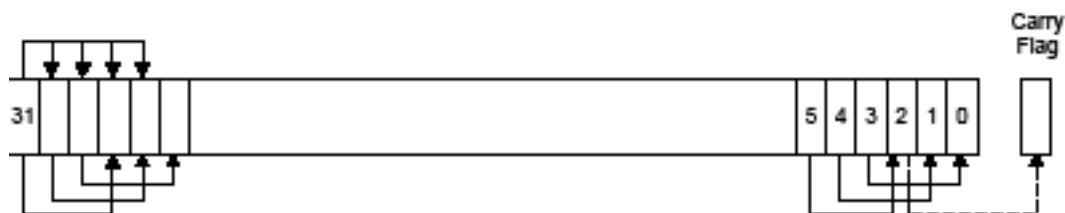
Figure 13-9. ASR #3
