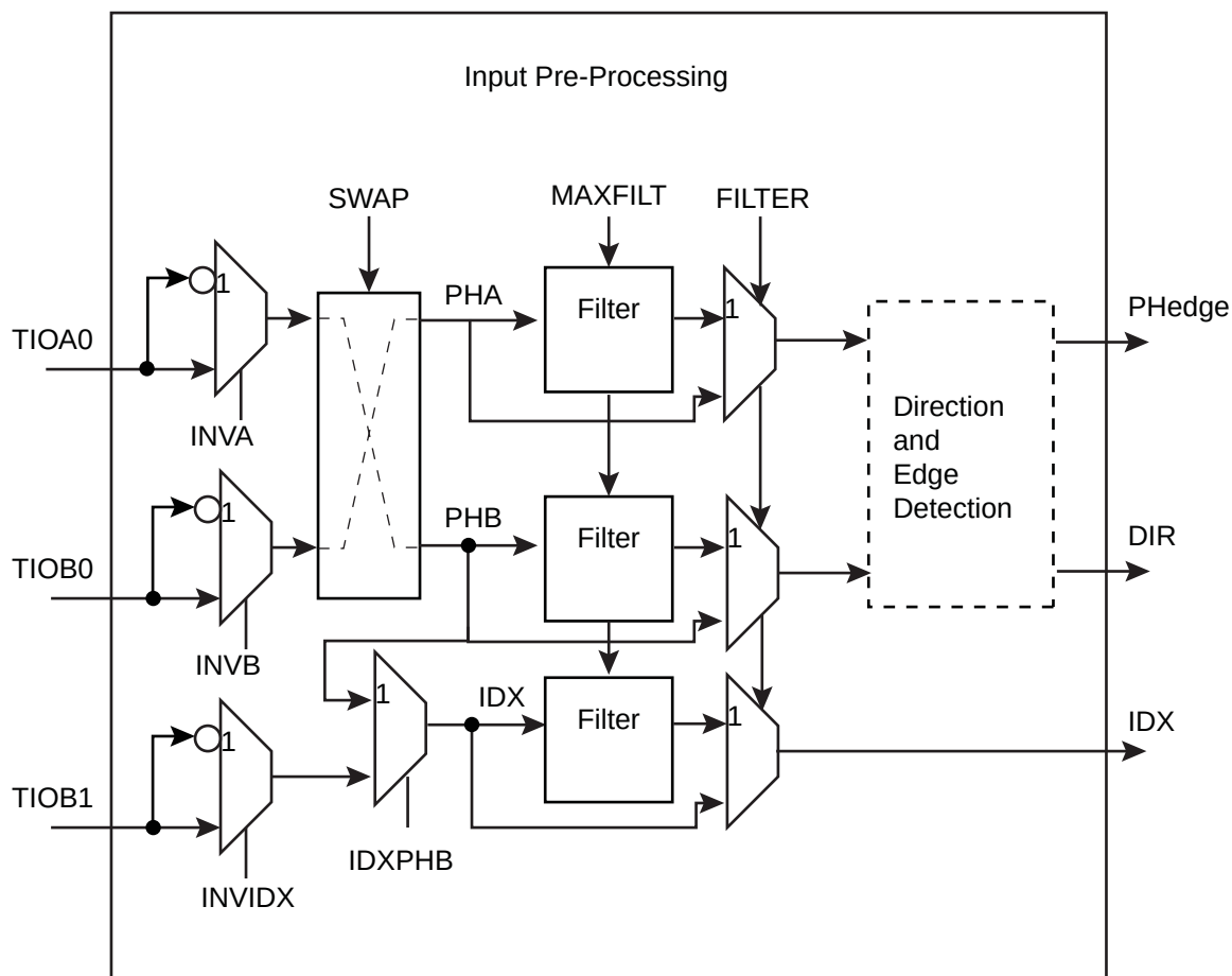
Figure 33-18. Input Stage
