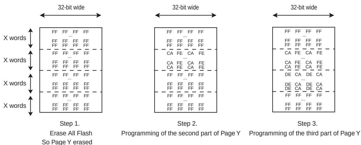
Figure 21-7. Example of Partial Page Programming
