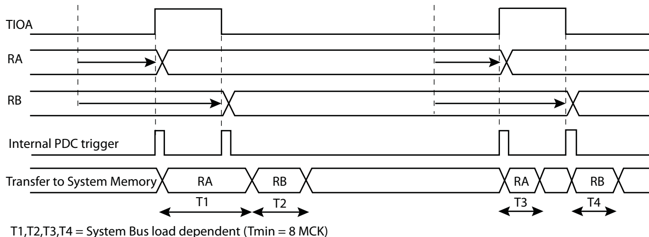
Figure 33-6. Example of transfer with PDC
