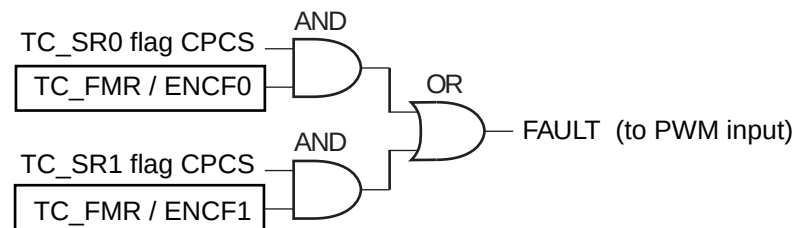
Figure 33-23.Fault Output Generation
