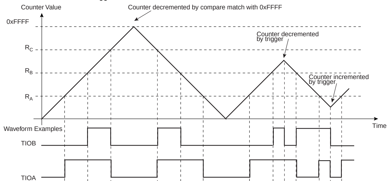
Figure 33-14. WAVSEL = 01 With Trigger
