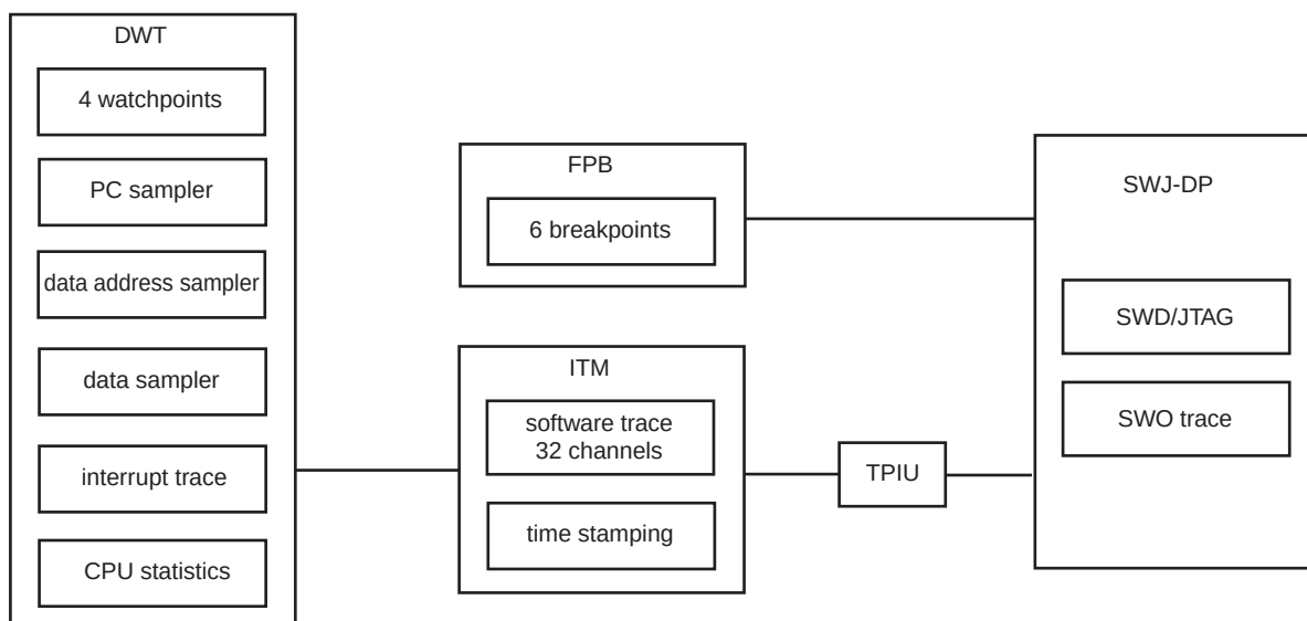
Figure 14-4. Debug Architecture
