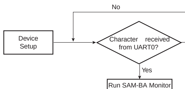
Figure 23-1. Boot Program Algorithm Flow Diagram
