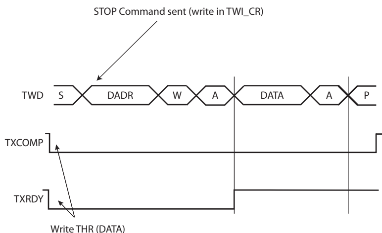
Figure 30-6. Master Write with One Data Byte
