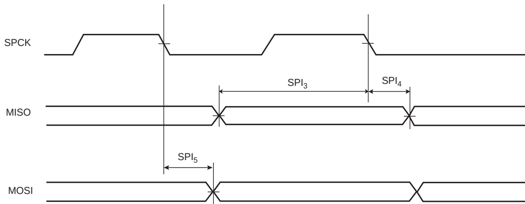
Figure 37-12. SPI Master Mode with (CPOL = 0 and NCPHA = 1) or (CPOL = 1 and NCPHA = 0)
