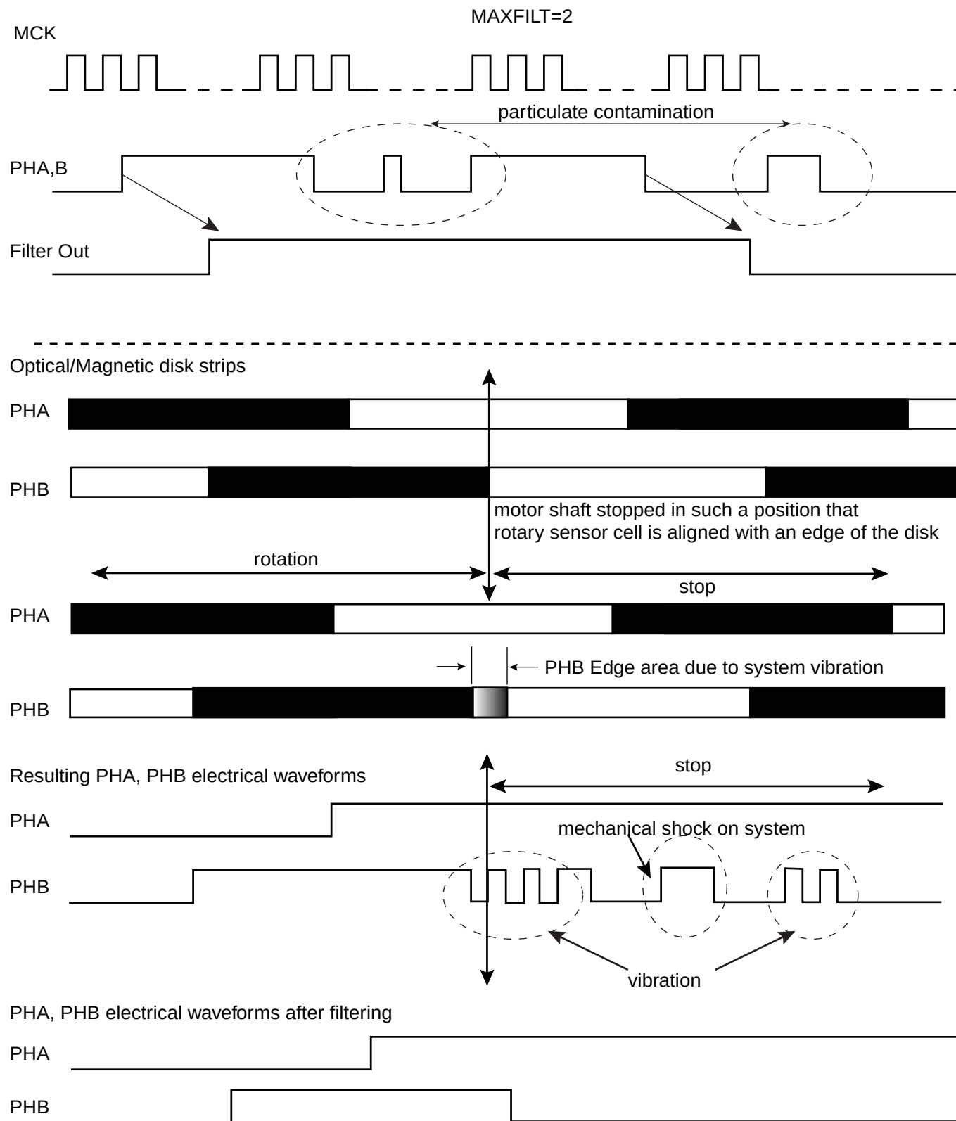
Figure 33-19. Filtering Examples
