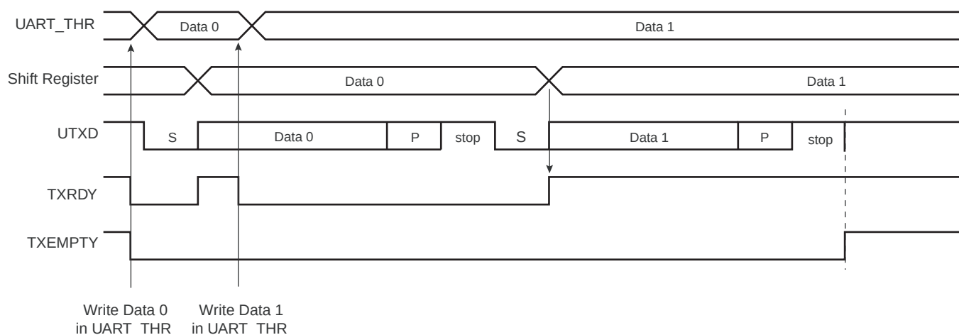
Figure 31-10. Transmitter Control
