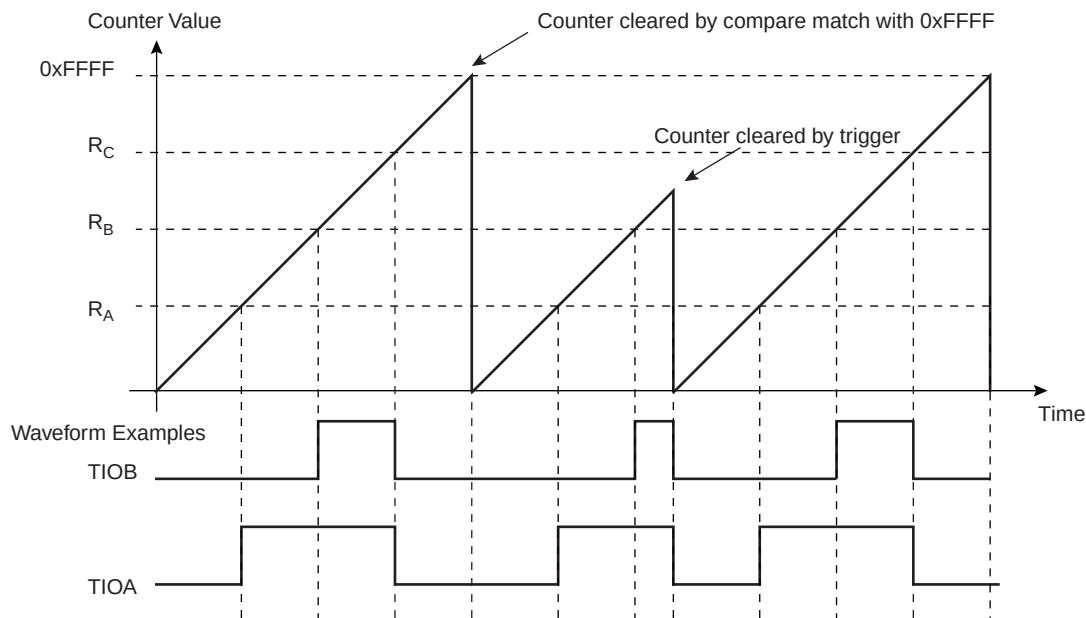
Figure 33-10. WAVSEL= 00 with trigger
