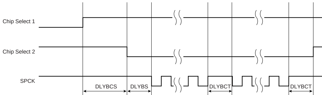
Figure 29-9. Programmable Delays
