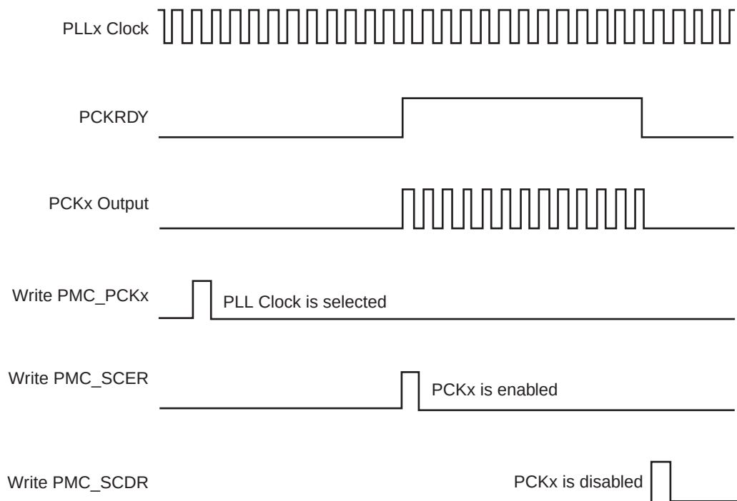
Figure 26-11. Programmable Clock Output Programming
