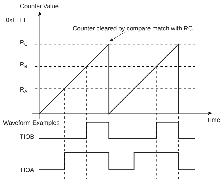
Figure 33-11. WAVSEL = 10 Without Trigger
