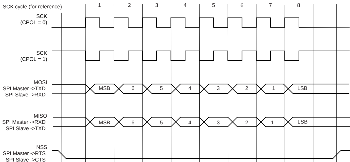
Figure 32-29. SPI Transfer Format (CPHA=0, 8 bits per transfer)
