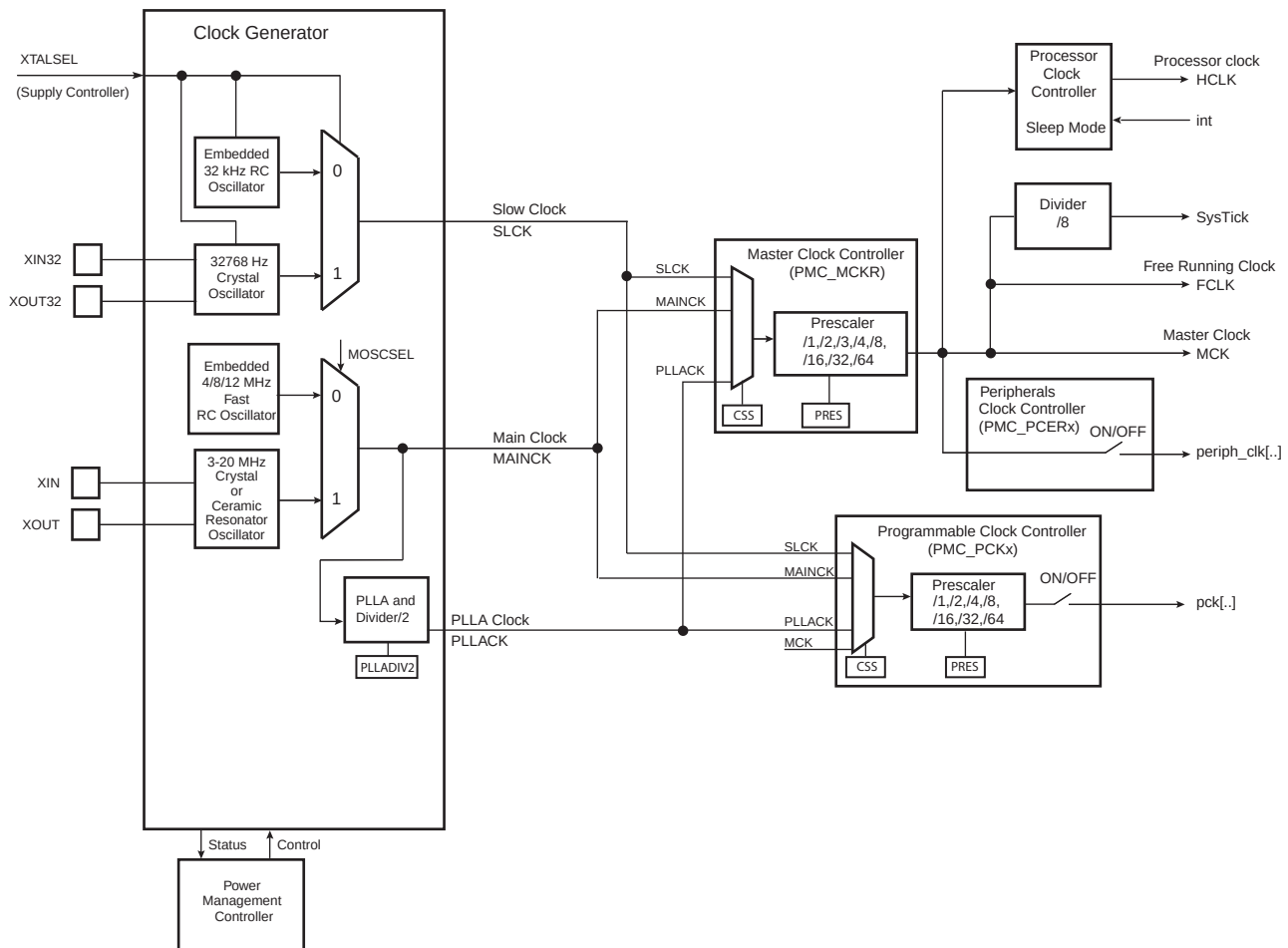
Figure 26-5. General Clock Block Diagram
